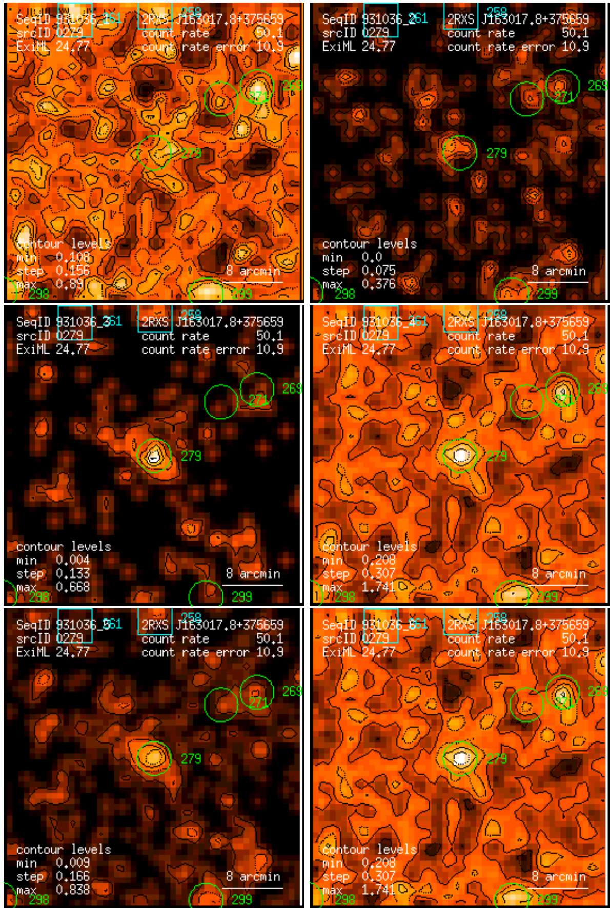
Figure 279: RASS 931036: detection 0279: band rate images, Gaussian filter: (1) PSPC channels 11 – 41, (2) 52 – 90, (3) 91 – 201, (4) 11 – 235, (5) 52 – 201, (6) 11 – 201. Broad band rates in counts/ks. Band rate contour levels in counts/ks/arcmin 2 .
