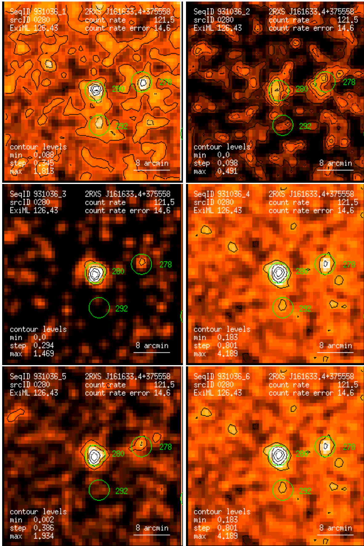
Figure 280: RASS 931036: detection 0280: band rate images, Gaussian filter: (1) PSPC channels 11 – 41, (2) 52 – 90, (3) 91 – 201, (4) 11 – 235, (5) 52 – 201, (6) 11 – 201. Broad band rates in counts/ks. Band rate contour levels in counts/ks/arcmin 2 .
