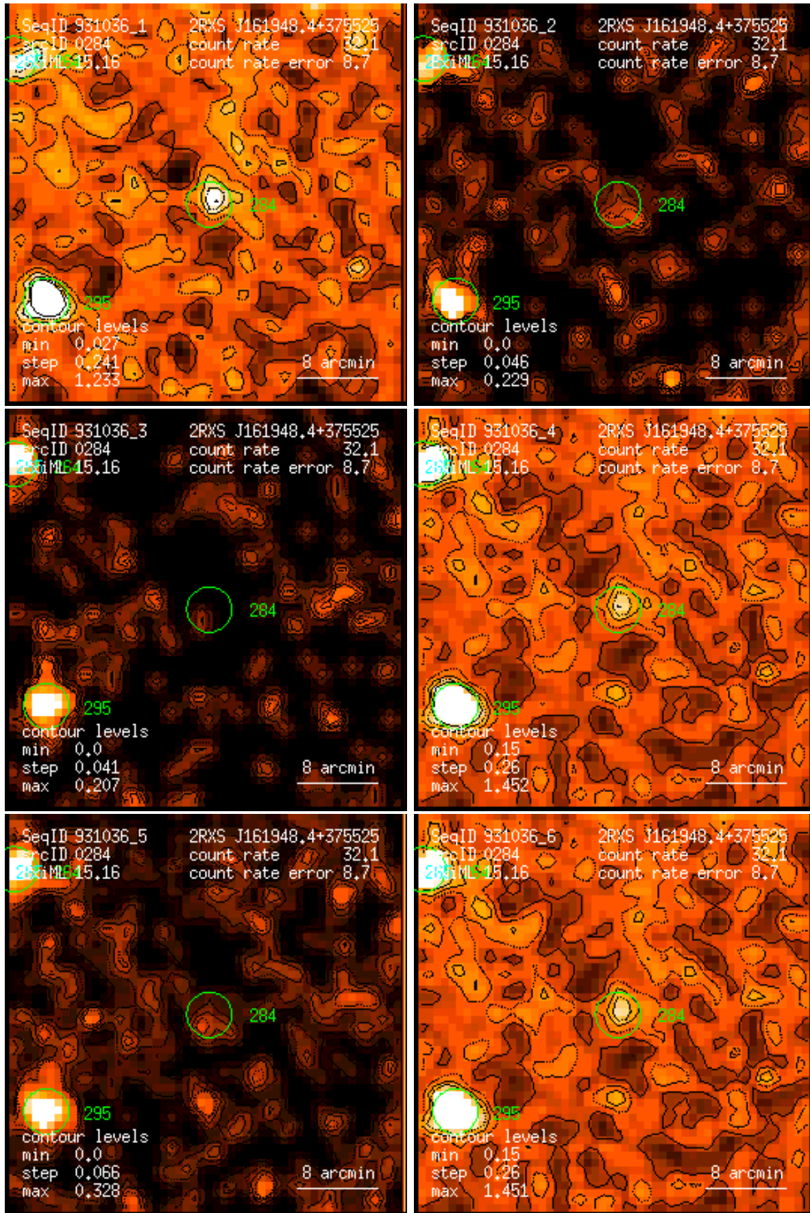
Figure 284: RASS 931036: detection 0284: band rate images, Gaussian filter: (1) PSPC channels 11 – 41, (2) 52 – 90, (3) 91 – 201, (4) 11 – 235, (5) 52 – 201, (6) 11 – 201. Broad band rates in counts/ks. Band rate contour levels in counts/ks/arcmin 2 .
