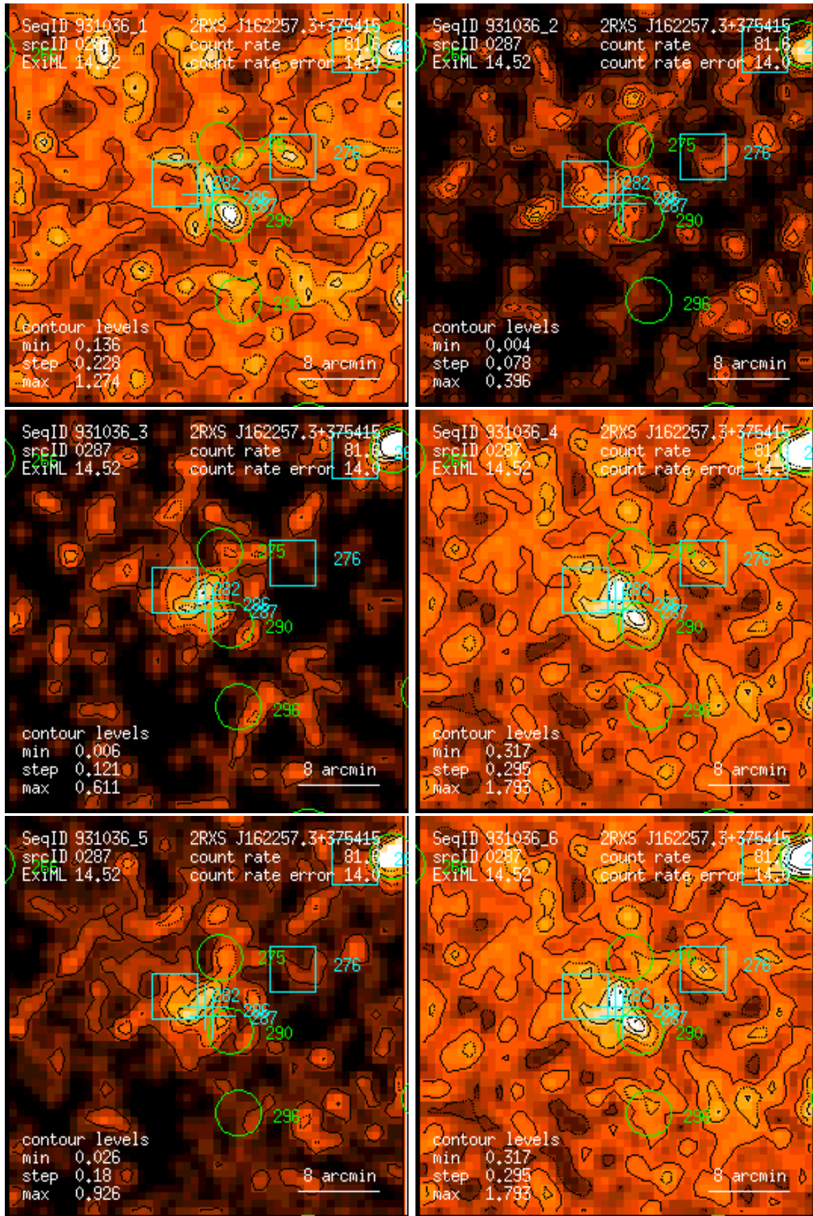
Figure 287: RASS 931036: detection 0287: band rate images, Gaussian filter: (1) PSPC channels 11 – 41, (2) 52 – 90, (3) 91 – 201, (4) 11 – 235, (5) 52 – 201, (6) 11 – 201. Broad band rates in counts/ks. Band rate contour levels in counts/ks/arcmin 2 .
