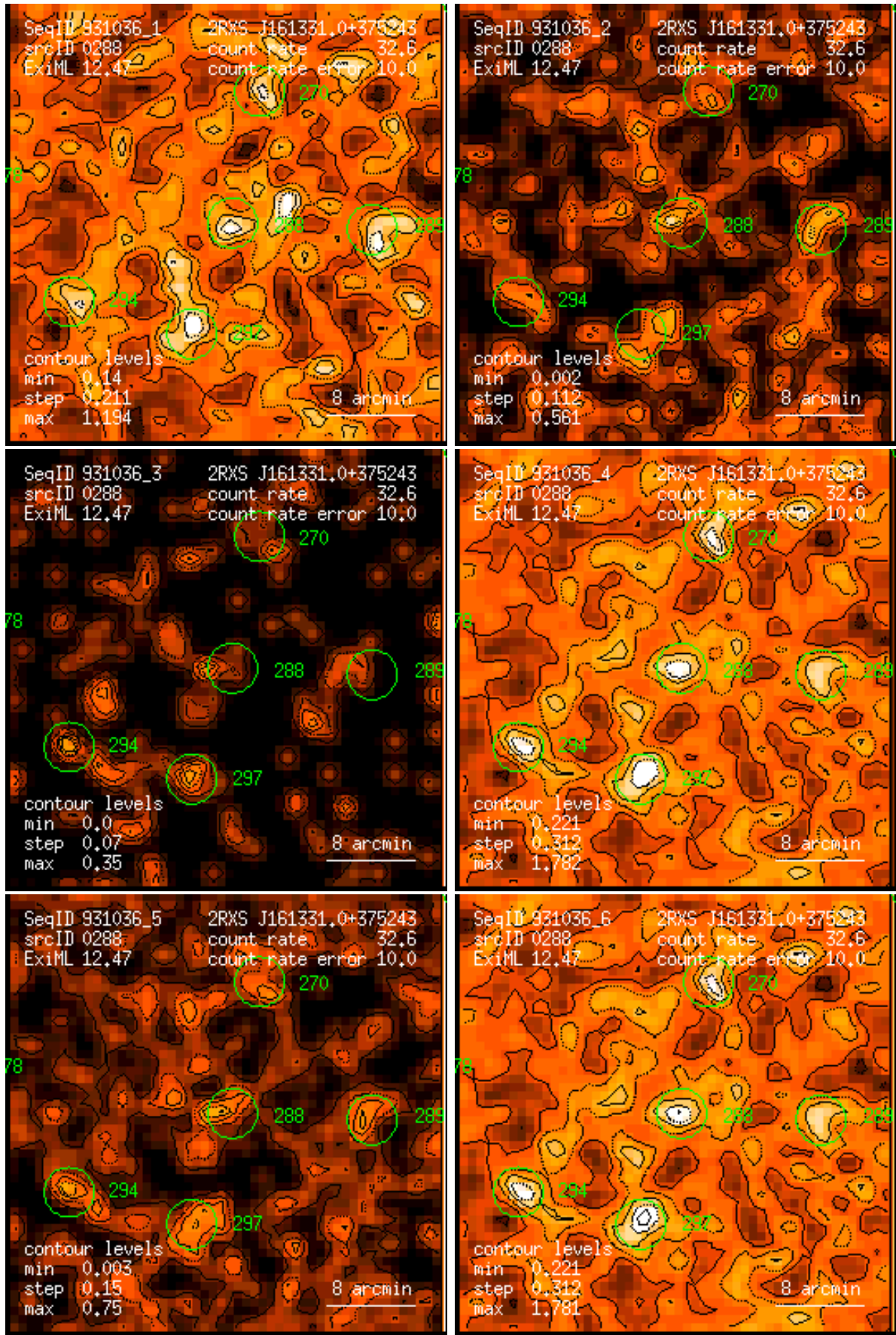
Figure 288: RASS 931036: detection 0288: band rate images, Gaussian filter: (1) PSPC channels 11 – 41, (2) 52 – 90, (3) 91 – 201, (4) 11 – 235, (5) 52 – 201, (6) 11 – 201. Broad band rates in counts/ks. Band rate contour levels in counts/ks/arcmin 2 .
