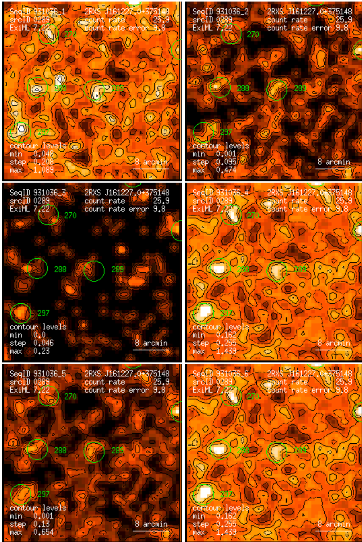
Figure 289: RASS 931036: detection 0289: band rate images, Gaussian filter: (1) PSPC channels 11 – 41, (2) 52 – 90, (3) 91 – 201, (4) 11 – 235, (5) 52 – 201, (6) 11 – 201. Broad band rates in counts/ks. Band rate contour levels in counts/ks/arcmin 2 .
