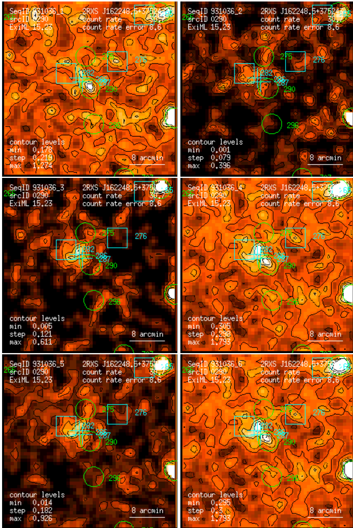
Figure 290: RASS 931036: detection 0290: band rate images, Gaussian filter: (1) PSPC channels 11 – 41, (2) 52 – 90, (3) 91 – 201, (4) 11 – 235, (5) 52 – 201, (6) 11 – 201. Broad band rates in counts/ks. Band rate contour levels in counts/ks/arcmin 2 .
