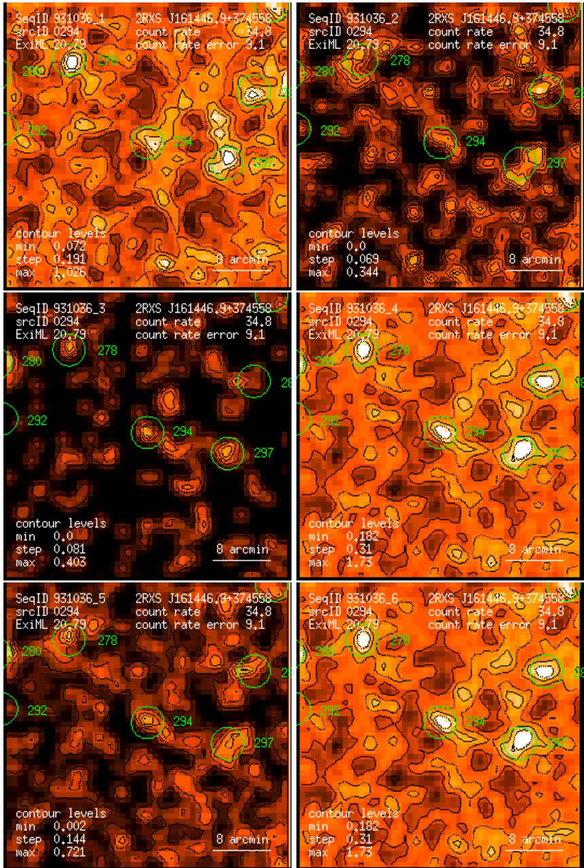
Figure 294: RASS 931036: detection 0294: band rate images, Gaussian filter: (1) PSPC channels 11 – 41, (2) 52 – 90, (3) 91 – 201, (4) 11 – 235, (5) 52 – 201, (6) 11 – 201. Broad band rates in counts/ks. Band rate contour levels in counts/ks/arcmin 2 .
