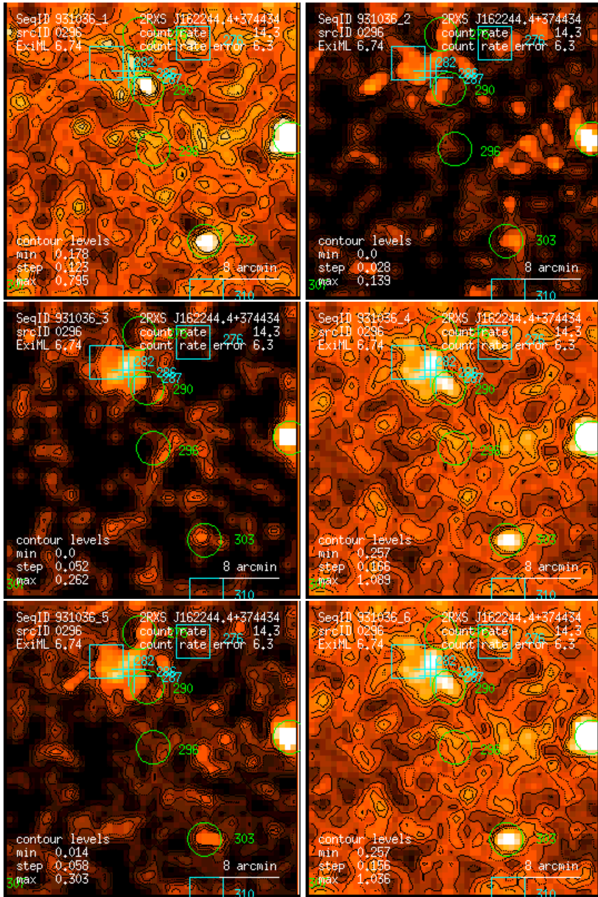
Figure 296: RASS 931036: detection 0296: band rate images, Gaussian filter: (1) PSPC channels 11 – 41, (2) 52 – 90, (3) 91 – 201, (4) 11 – 235, (5) 52 – 201, (6) 11 – 201. Broad band rates in counts/ks. Band rate contour levels in counts/ks/arcmin 2 .
