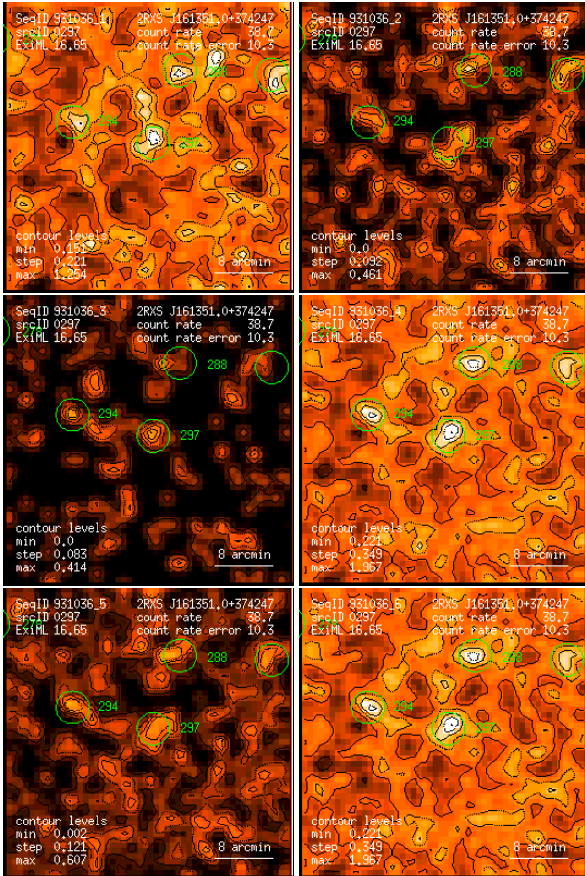
Figure 297: RASS 931036: detection 0297: band rate images, Gaussian filter: (1) PSPC channels 11 – 41, (2) 52 – 90, (3) 91 – 201, (4) 11 – 235, (5) 52 – 201, (6) 11 – 201. Broad band rates in counts/ks. Band rate contour levels in counts/ks/arcmin 2 .
