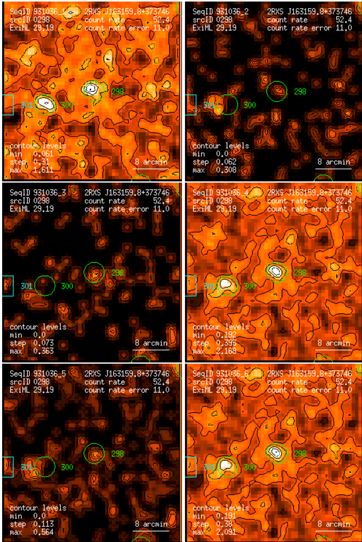
Figure 298: RASS 931036: detection 0298: band rate images, Gaussian filter: (1) PSPC channels 11 – 41, (2) 52 – 90, (3) 91 – 201, (4) 11 – 235, (5) 52 – 201, (6) 11 – 201. Broad band rates in counts/ks. Band rate contour levels in counts/ks/arcmin 2 .
