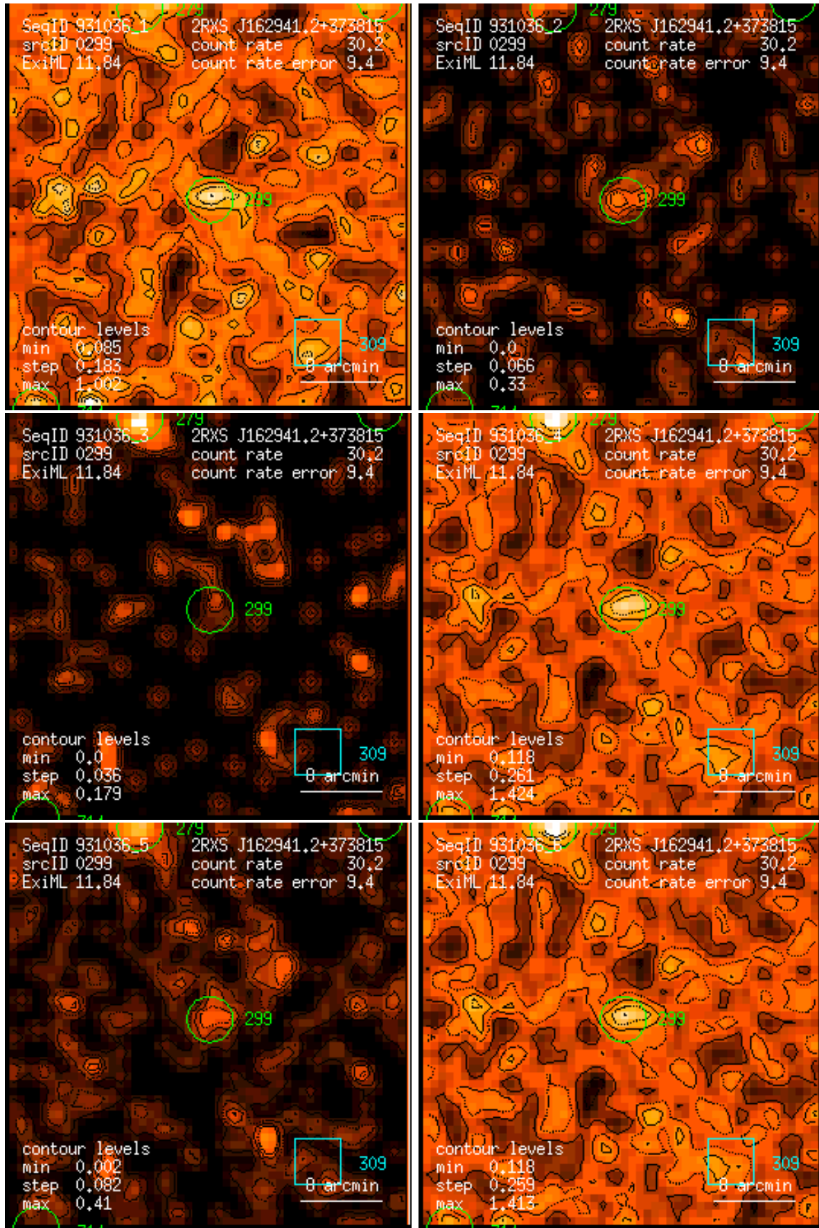
Figure 299: RASS 931036: detection 0299: band rate images, Gaussian filter: (1) PSPC channels 11 – 41, (2) 52 – 90, (3) 91 – 201, (4) 11 – 235, (5) 52 – 201, (6) 11 – 201. Broad band rates in counts/ks. Band rate contour levels in counts/ks/arcmin 2 .
