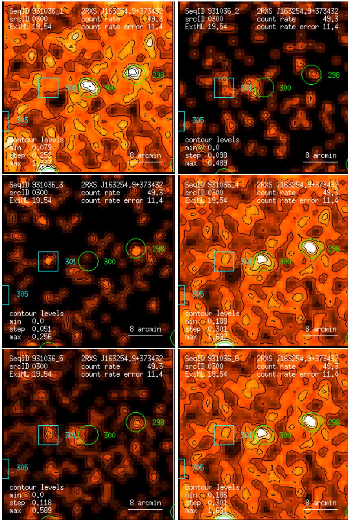
Figure 300: RASS 931036: detection 0300: band rate images, Gaussian filter: (1) PSPC channels 11 – 41, (2) 52 – 90, (3) 91 – 201, (4) 11 – 235, (5) 52 – 201, (6) 11 – 201. Broad band rates in counts/ks. Band rate contour levels in counts/ks/arcmin 2 .
