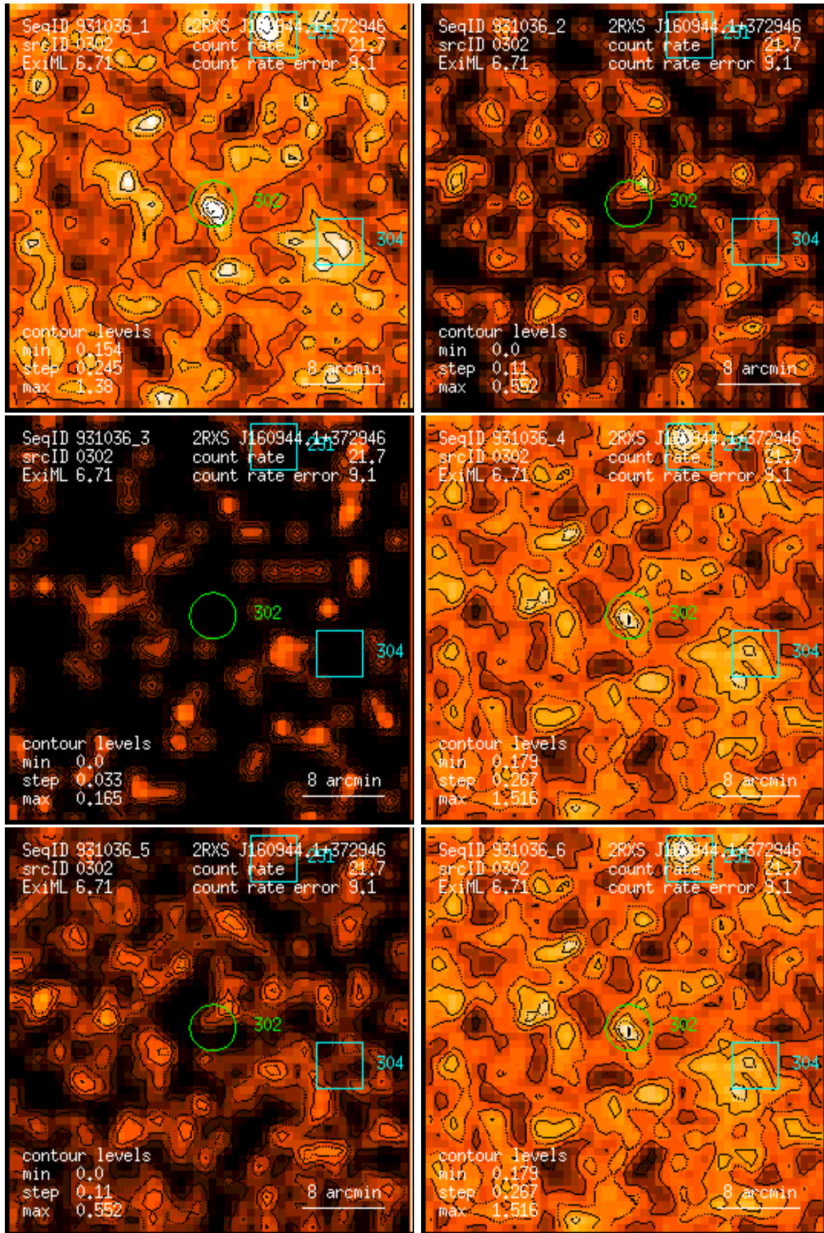
Figure 302: RASS 931036: detection 0302: band rate images, Gaussian filter: (1) PSPC channels 11 – 41, (2) 52 – 90, (3) 91 – 201, (4) 11 – 235, (5) 52 – 201, (6) 11 – 201. Broad band rates in counts/ks. Band rate contour levels in counts/ks/arcmin 2 .
