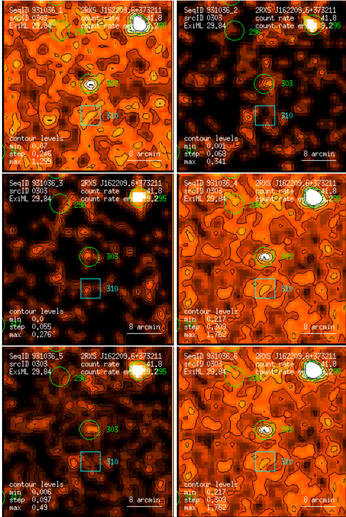
Figure 303: RASS 931036: detection 0303: band rate images, Gaussian filter: (1) PSPPC channels 11 – 41, (2) 52 – 90, (3) 91 – 201, (4) 11 – 235, (5) 52 – 201, (6) 11 – 201. Broad band rates in counts/ks. Band rate contour levels in counts/ks/arcmin 2 .
