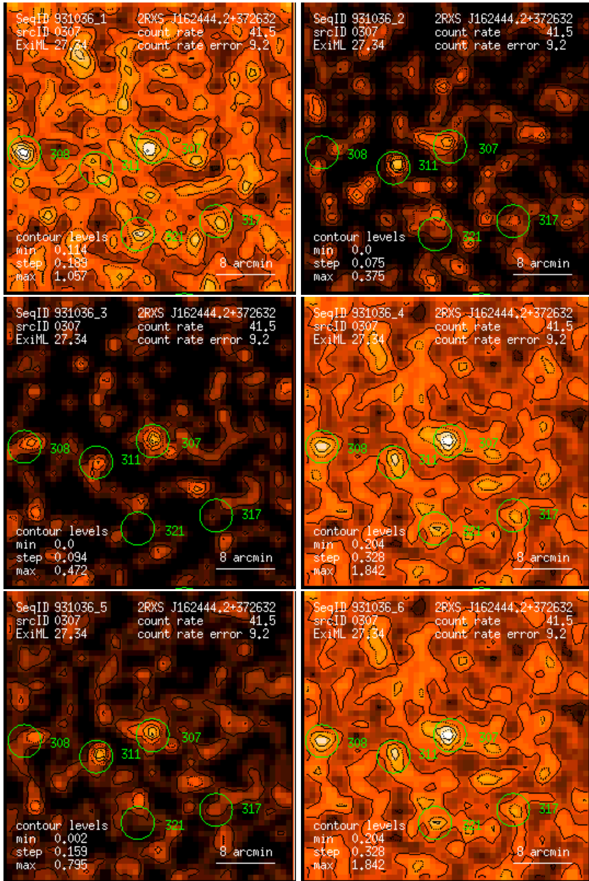
Figure 307: RASS 931036: detection 0307: band rate images, Gaussian filter: (1) PSPC channels 11 – 41, (2) 52 – 90, (3) 91 – 201, (4) 11 – 235, (5) 52 – 201, (6) 11 – 201. Broad band rates in counts/ks. Band rate contour levels in counts/ks/arcmin 2 .
