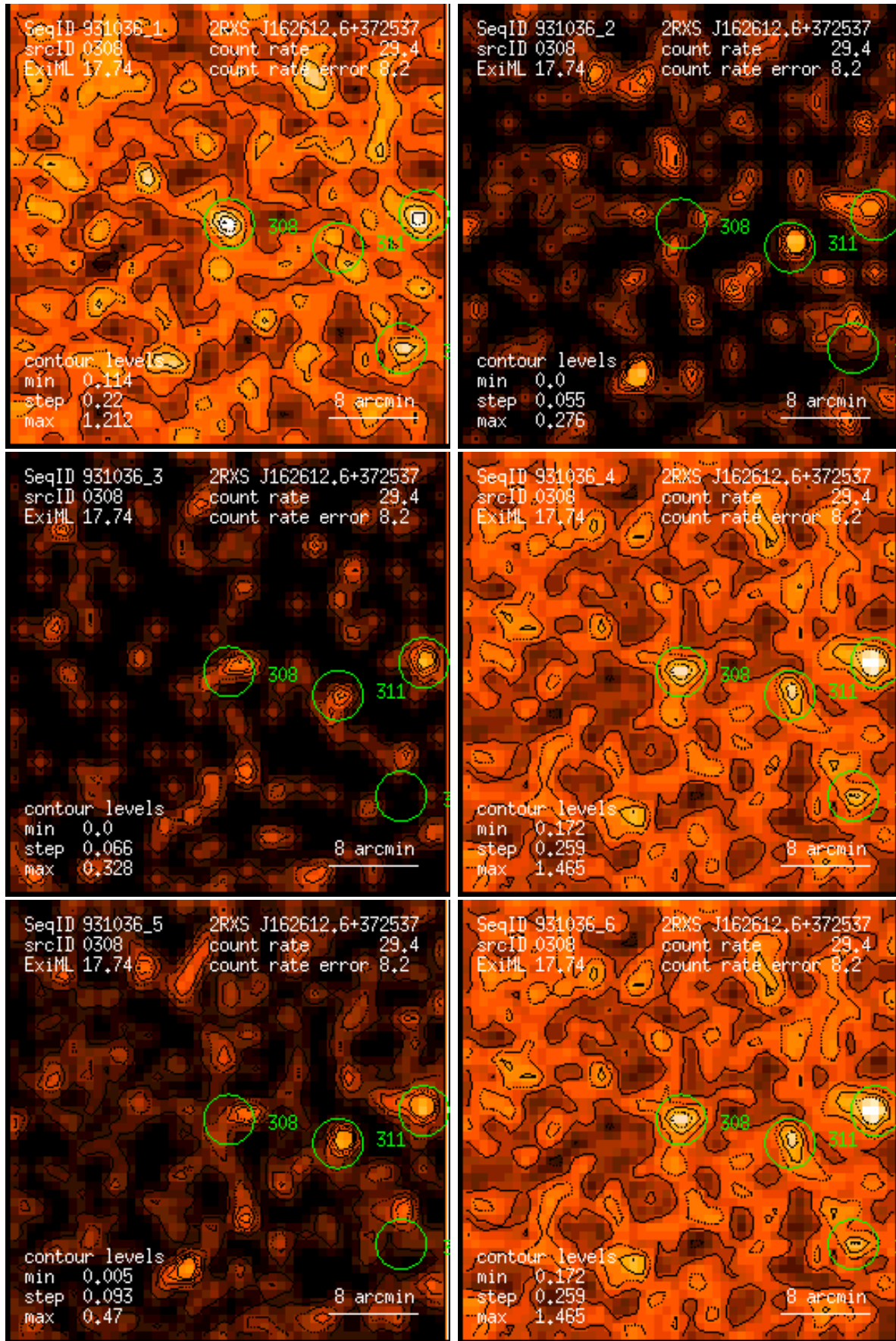
Figure 308: RASS 931036: detection 0308: band rate images, Gaussian filter: (1) PSPC channels 11 – 41, (2) 52 – 90, (3) 91 – 201, (4) 11 – 235, (5) 52 – 201, (6) 11 – 201. Broad band rates in counts/ks. Band rate contour levels in counts/ks/arcmin 2 .
