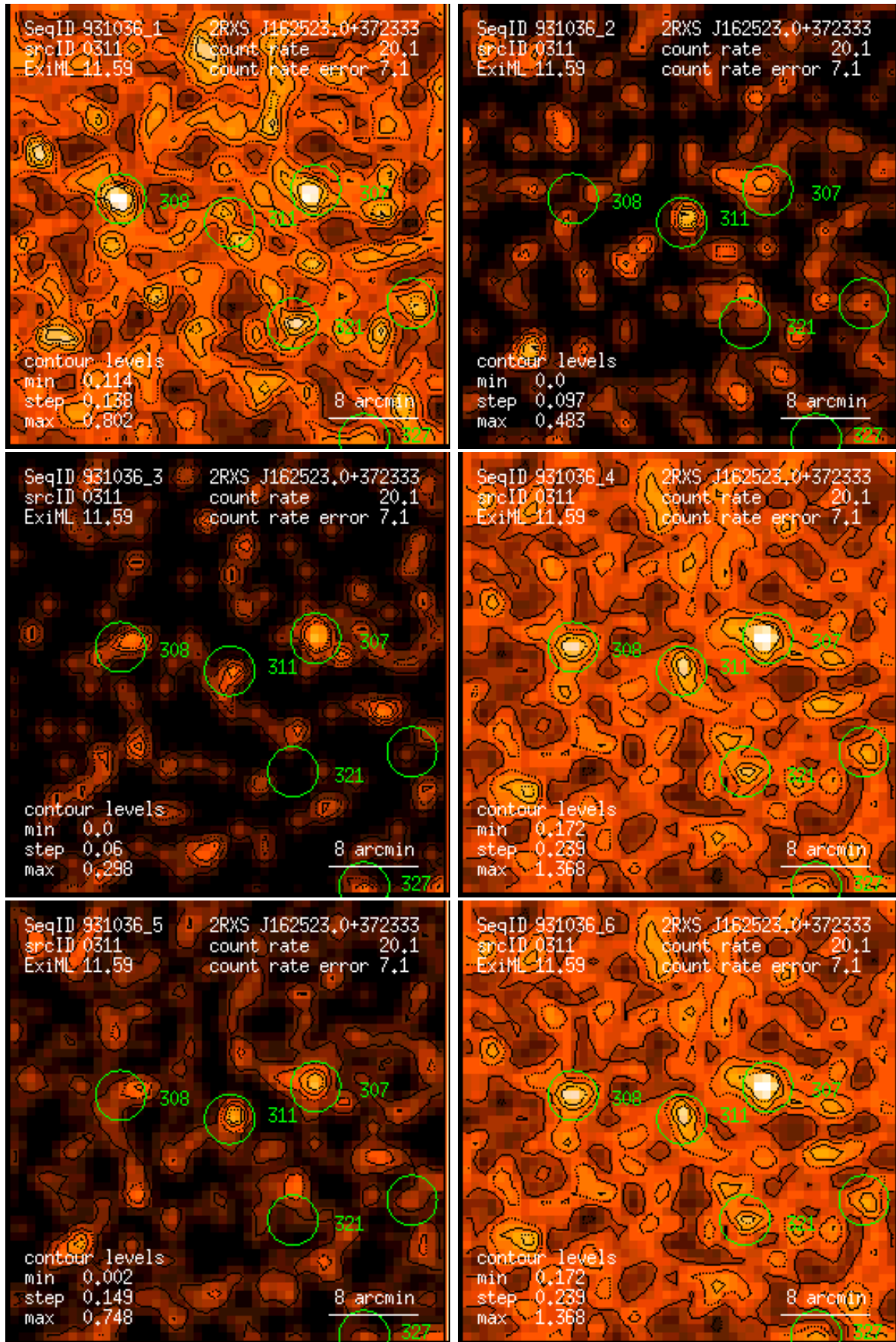
Figure 311: RASS 931036: detection 0311: band rate images, Gaussian filter: (1) PSPC channels 11 – 41, (2) 52 – 90, (3) 91 – 201, (4) 11 – 235, (5) 52 – 201, (6) 11 – 201. Broad band rates in counts/ks. Band rate contour levels in counts/ks/arcmin 2 .
