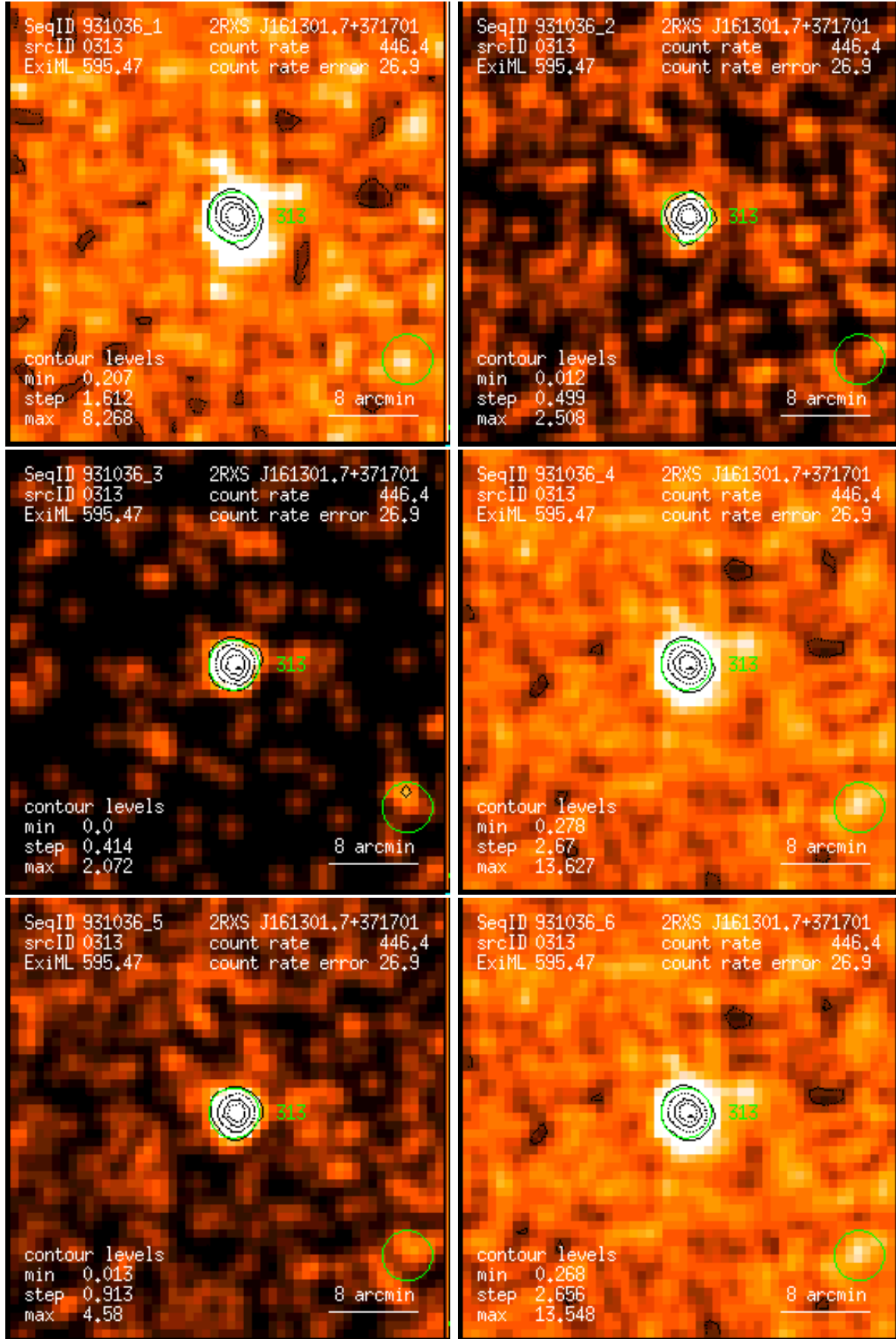
Figure 313: RASS 931036: detection 0313: band rate images, Gaussian filter: (1) PSPC channels 11 – 41, (2) 52 – 90, (3) 91 – 201, (4) 11 – 235, (5) 52 – 201, (6) 11 – 201. Broad band rates in counts/ks. Band rate contour levels in counts/ks/arcmin 2 .
