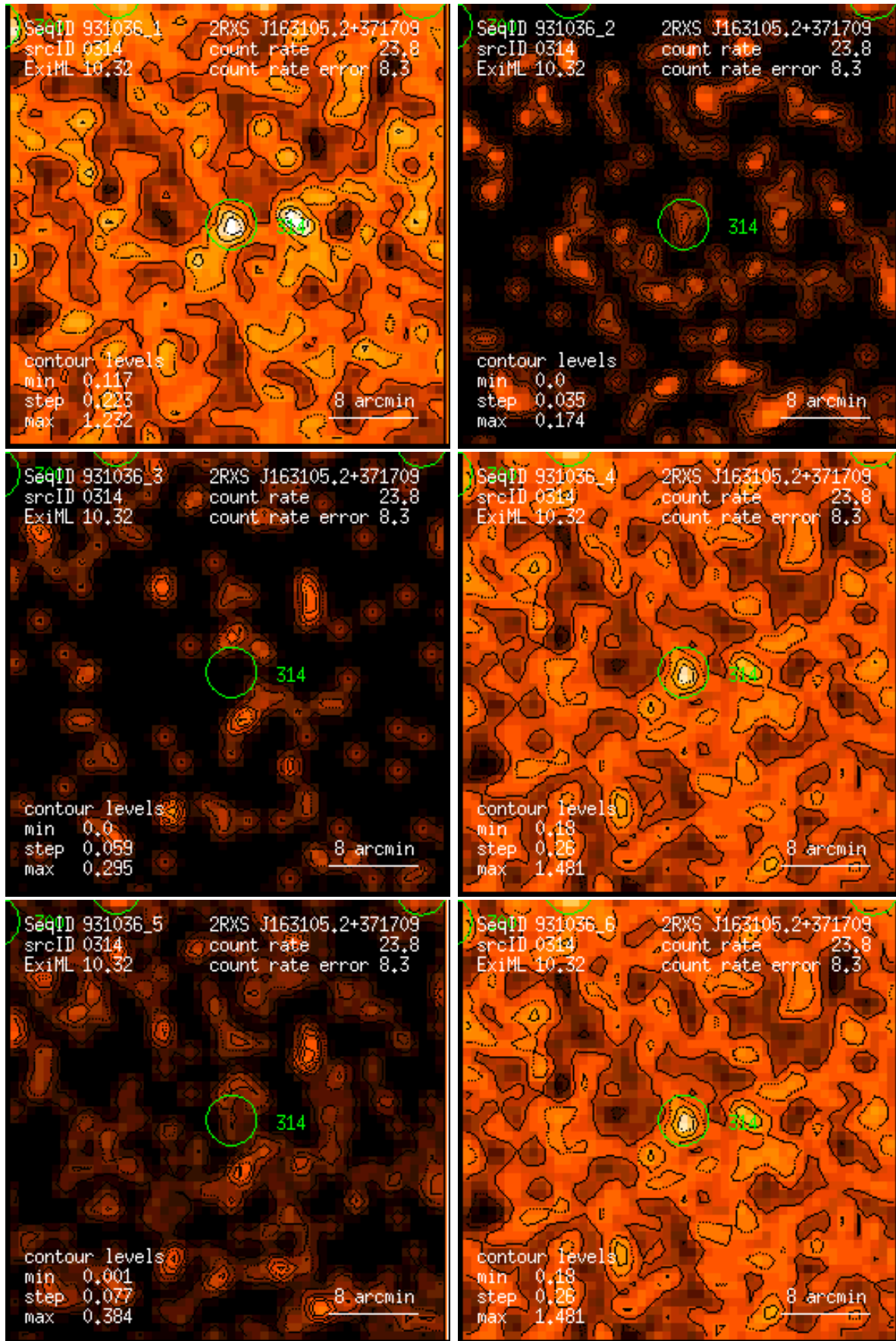
Figure 314: RASS 931036: detection 0314: band rate images, Gaussian filter: (1) PSPC channels 11 – 41, (2) 52 – 90, (3) 91 – 201, (4) 11 – 235, (5) 52 – 201, (6) 11 – 201. Broad band rates in counts/ks. Band rate contour levels in counts/ks/arcmin 2 .
