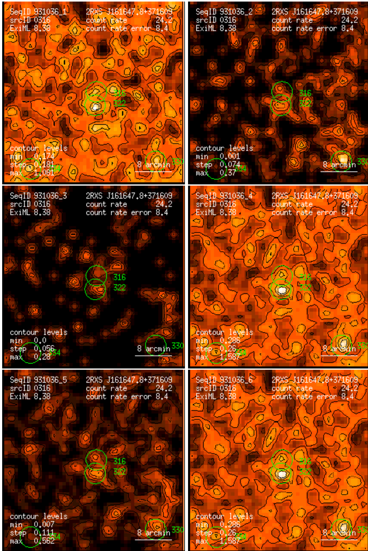
Figure 316: RASS 931036: detection 0316: band rate images, Gaussian filter: (1) PSPC channels 11 – 41, (2) 52 – 90, (3) 91 – 201, (4) 11 – 235, (5) 52 – 201, (6) 11 – 201. Broad band rates in counts/ks. Band rate contour levels in counts/ks/arcmin 2 .
