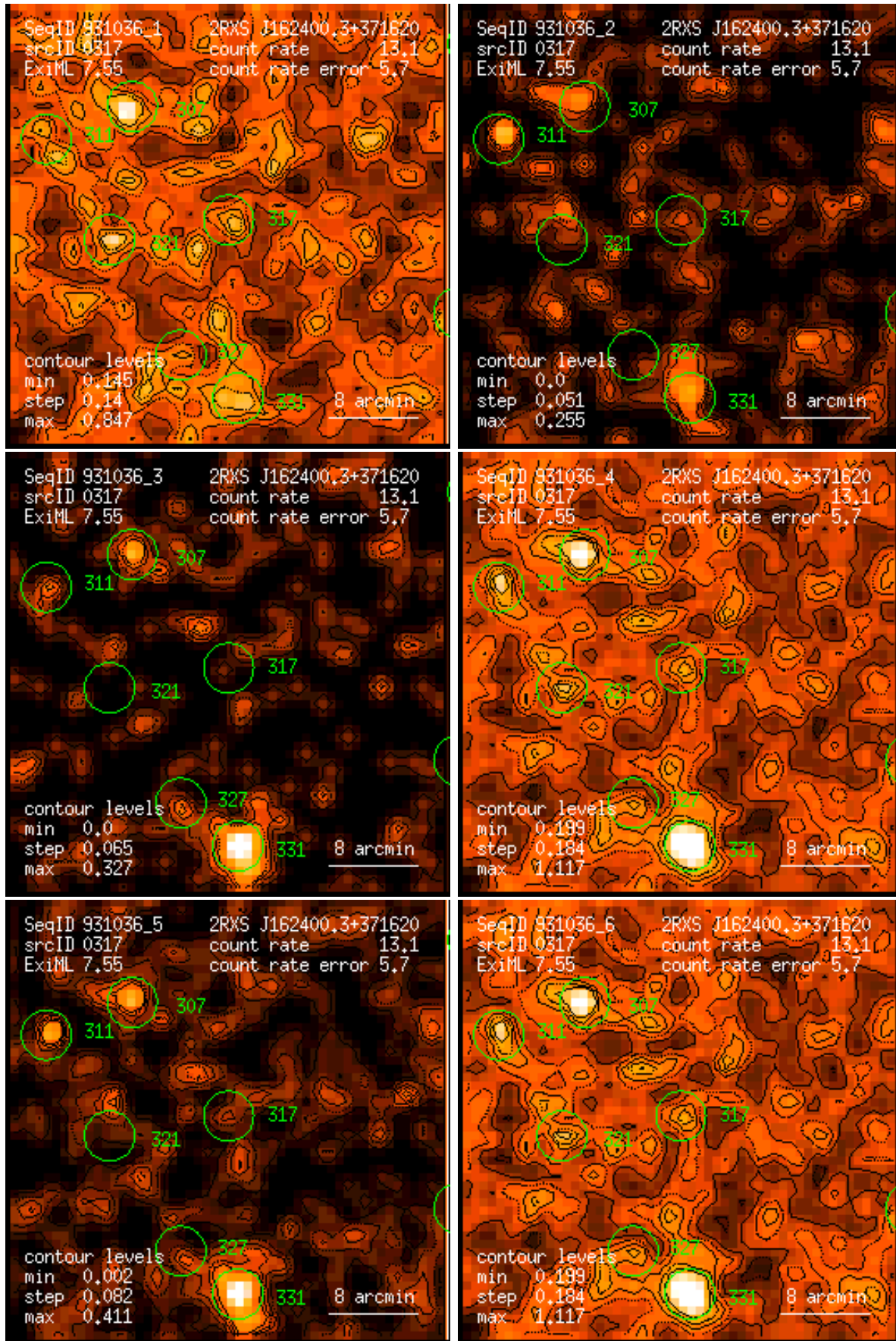
Figure 317: RASS 931036: detection 0317: band rate images, Gaussian filter: (1) PSPC channels 11 – 41, (2) 52 – 90, (3) 91 – 201, (4) 11 – 235, (5) 52 – 201, (6) 11 – 201. Broad band rates in counts/ks. Band rate contour levels in counts/ks/arcmin 2 .
