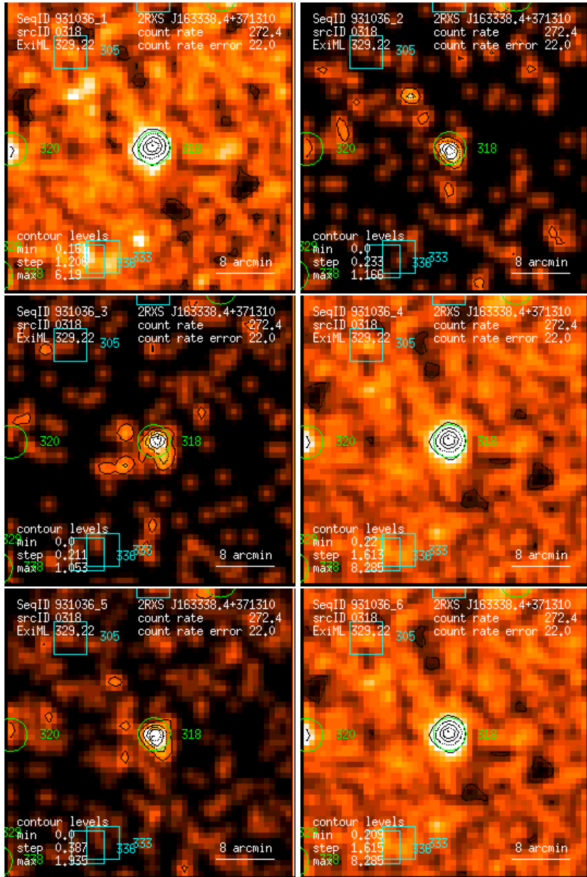
Figure 318: RASS 931036: detection 0318: band rate images, Gaussian filter: (1) PSPC channels 11 – 41, (2) 52 – 90, (3) 91 – 201, (4) 11 – 235, (5) 52 – 201, (6) 11 – 201. Broad band rates in counts/ks. Band rate contour levels in counts/ks/arcmin 2 .
