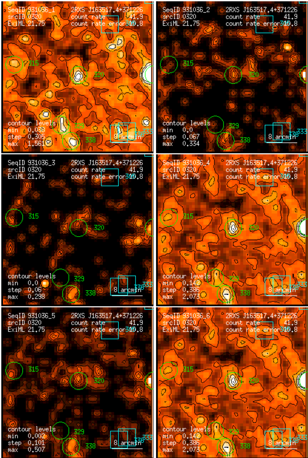
Figure 320: RASS 931036: detection 0320: band rate images, Gaussian filter: (1) PSPC channels 11 – 41, (2) 52 – 90, (3) 91 – 201, (4) 11 – 235, (5) 52 – 201, (6) 11 – 201. Broad band rates in counts/ks. Band rate contour levels in counts/ks/arcmin 2 .
