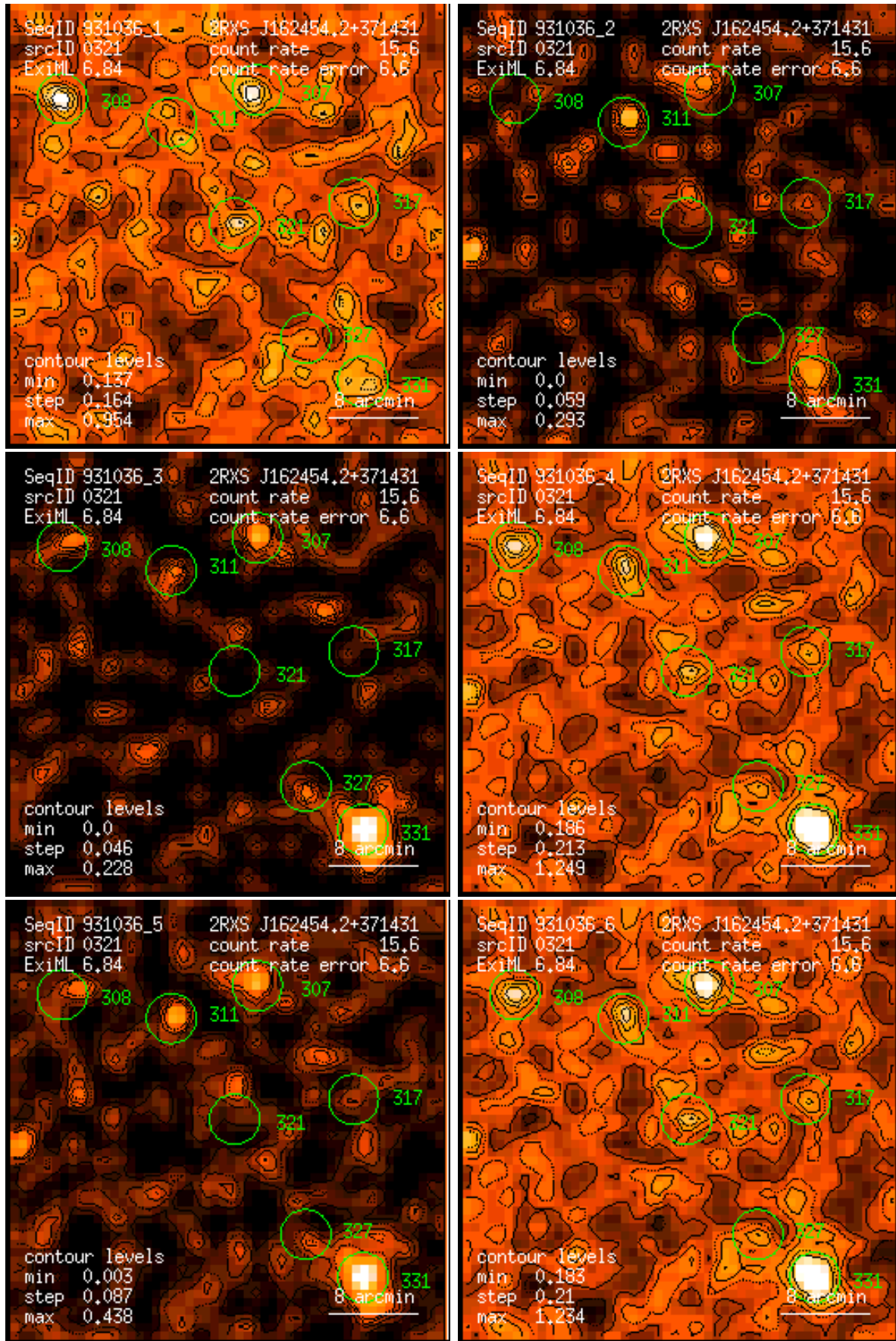
Figure 321: RASS 931036: detection 0321: band rate images, Gaussian filter: (1) PSPC channels 11 – 41, (2) 52 – 90, (3) 91 – 201, (4) 11 – 235, (5) 52 – 201, (6) 11 – 201. Broad band rates in counts/ks. Band rate contour levels in counts/ks/arcmin 2 .
