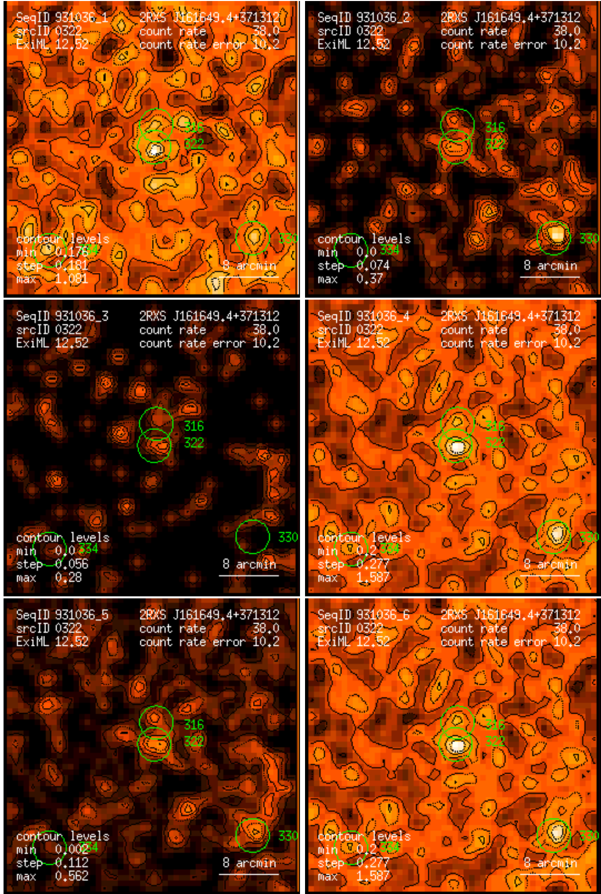
Figure 322: RASS 931036: detection 0322: band rate images, Gaussian filter: (1) PSPC channels 11 – 41, (2) 52 – 90, (3) 91 – 201, (4) 11 – 235, (5) 52 – 201, (6) 11 – 201. Broad band rates in counts/ks. Band rate contour levels in counts/ks/arcmin 2 .
