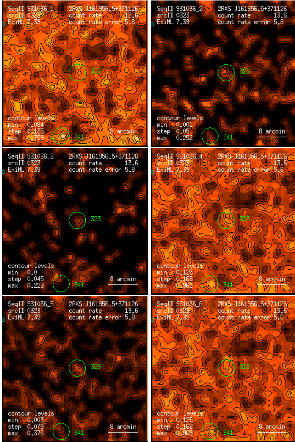
Figure 323: RASS 931036: detection 0323: band rate images, Gaussian filter: (1) PSPC channels 11 – 41, (2) 52 – 90, (3) 91 – 201, (4) 11 – 235, (5) 52 – 201, (6) 11 – 201. Broad band rates in counts/ks. Band rate contour levels in counts/ks/arcmin 2 .
