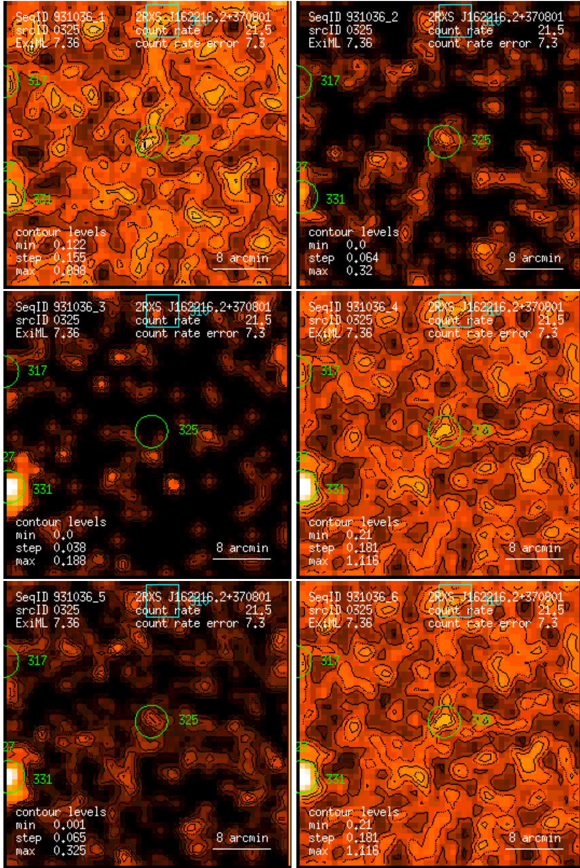
Figure 325: RASS 931036: detection 0325: band rate images, Gaussian filter: (1) PSPC channels 11 – 41, (2) 52 – 90, (3) 91 – 201, (4) 11 – 235, (5) 52 – 201, (6) 11 – 201. Broad band rates in counts/ks. Band rate contour levels in counts/ks/arcmin 2 .
