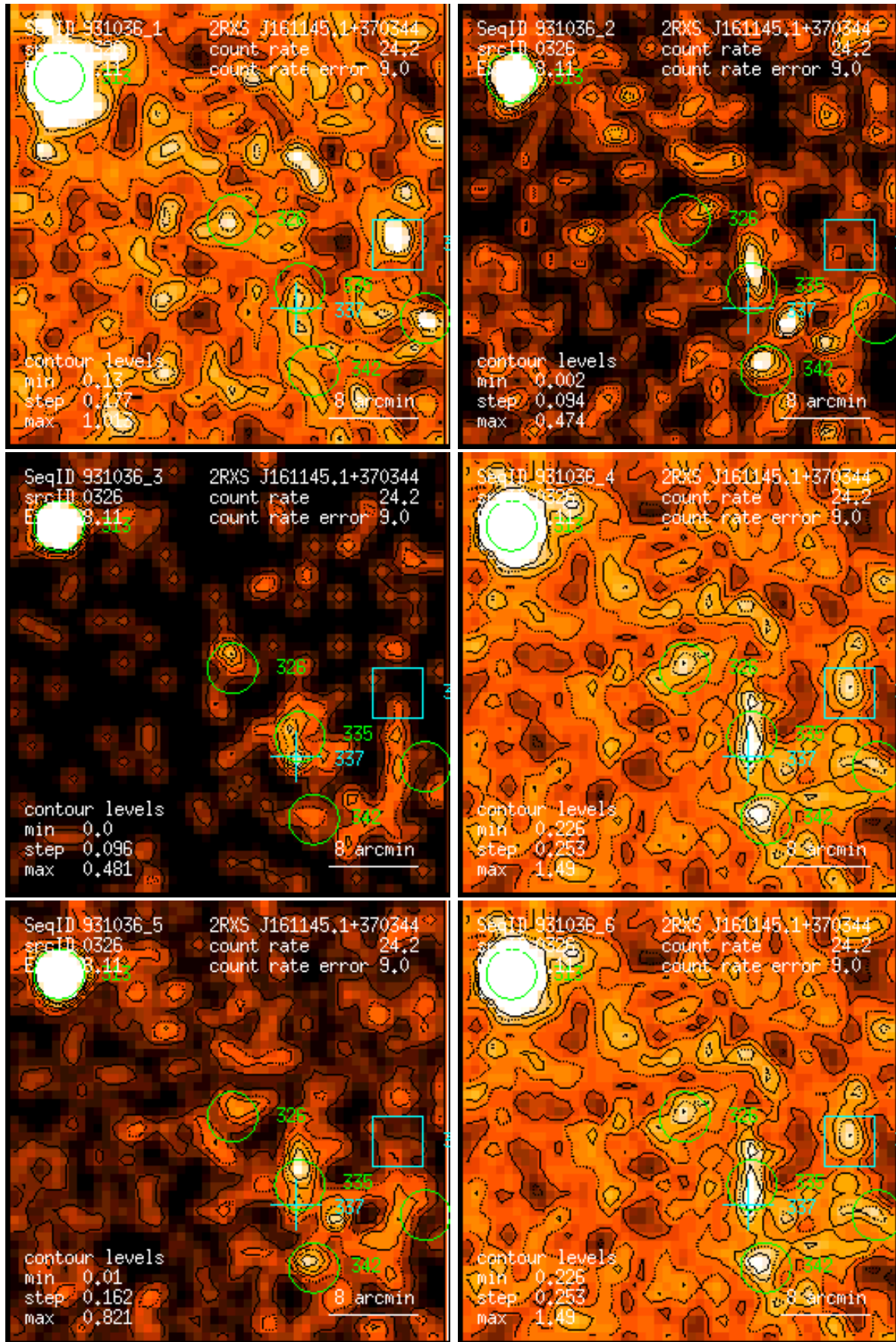
Figure 326: RASS 931036: detection 0326: band rate images, Gaussian filter: (1) PSPC channels 11 – 41, (2) 52 – 90, (3) 91 – 201, (4) 11 – 235, (5) 52 – 201, (6) 11 – 201. Broad band rates in counts/ks. Band rate contour levels in counts/ks/arcmin 2 .
