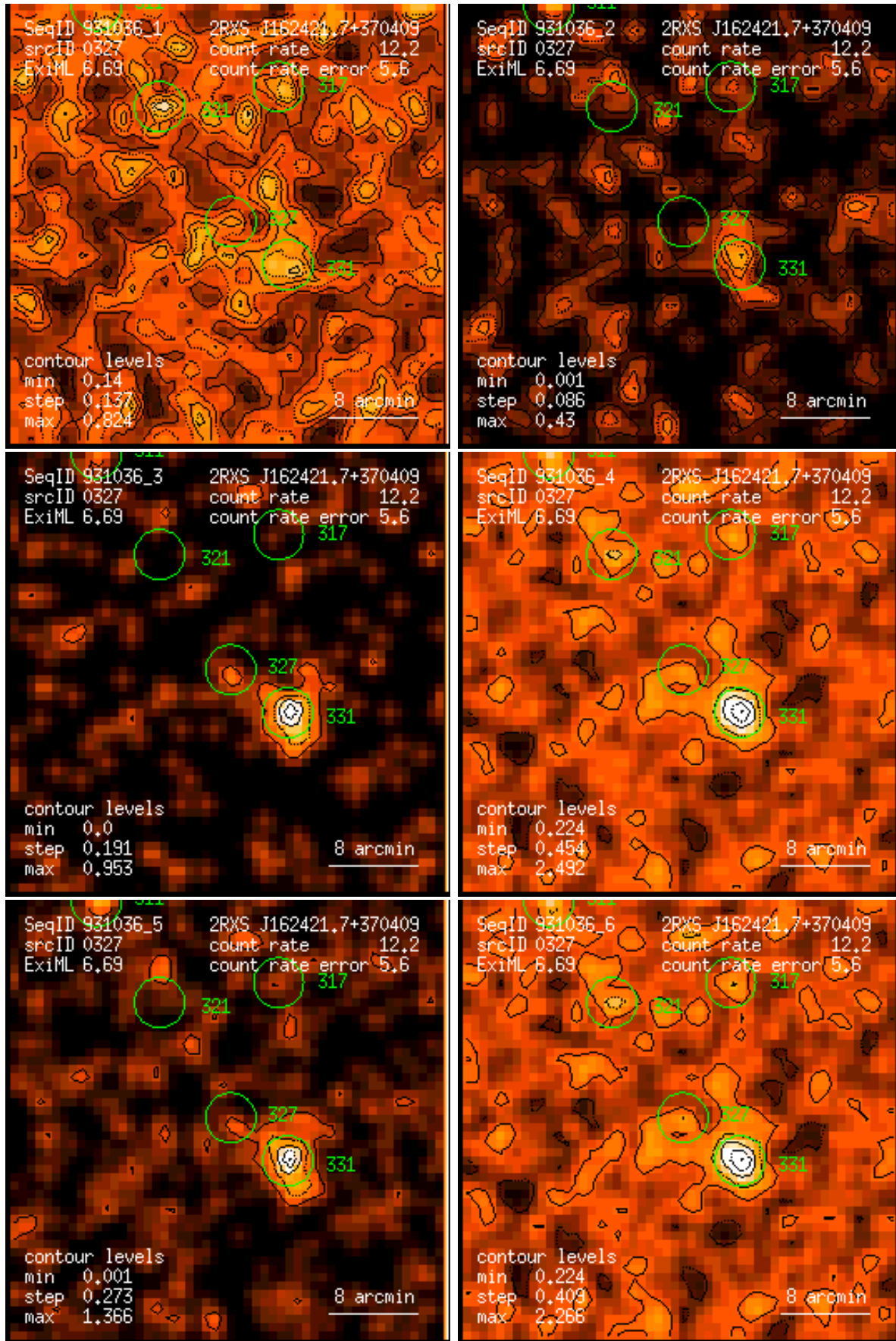
Figure 327: RASS 931036: detection 0327: band rate images, Gaussian filter: (1) PSPC channels 11 – 41, (2) 52 – 90, (3) 91 – 201, (4) 11 – 235, (5) 52 – 201, (6) 11 – 201. Broad band rates in counts/ks. Band rate contour levels in counts/ks/arcmin 2 .
