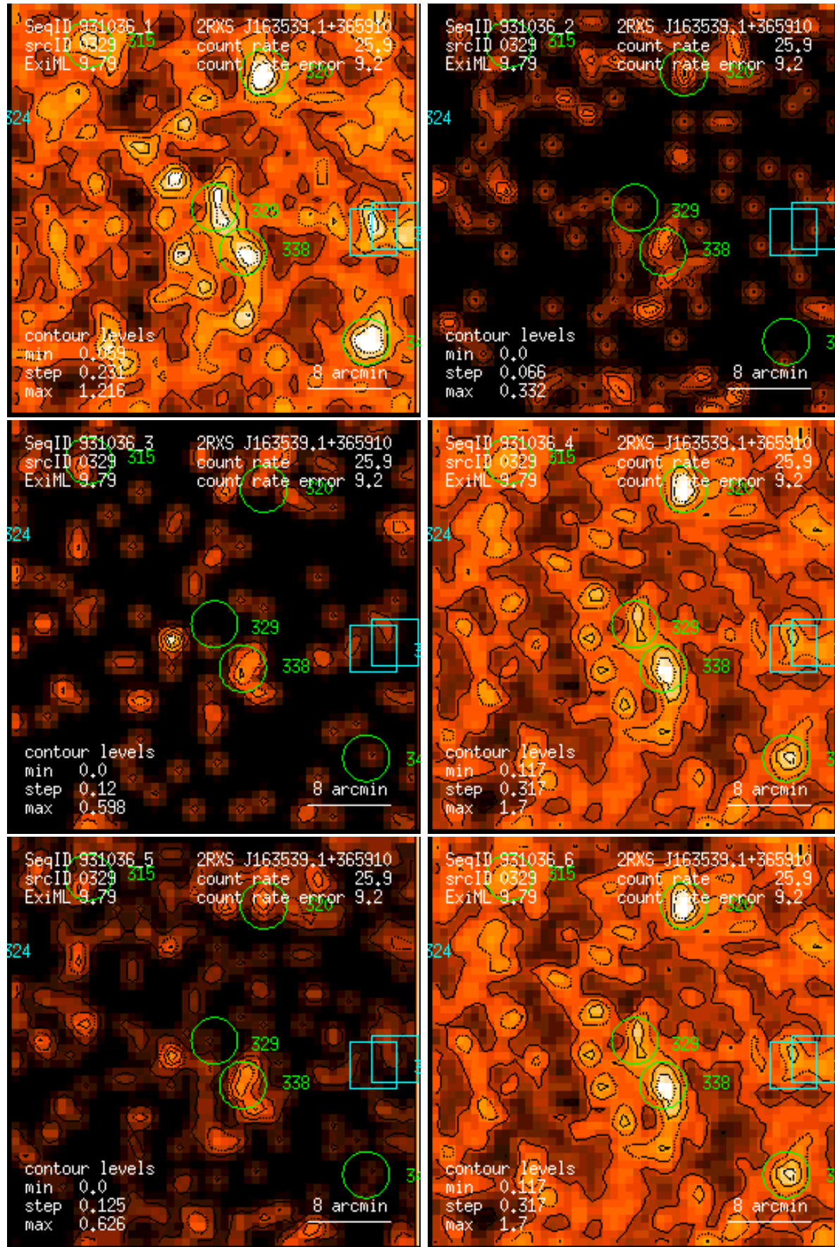
Figure 329: RASS 931036: detection 0329: band rate images, Gaussian filter: (1) PSPC channels 11 – 41, (2) 52 – 90, (3) 91 – 201, (4) 11 – 235, (5) 52 – 201, (6) 11 – 201. Broad band rates in counts/ks. Band rate contour levels in counts/ks/arcmin 2 .
