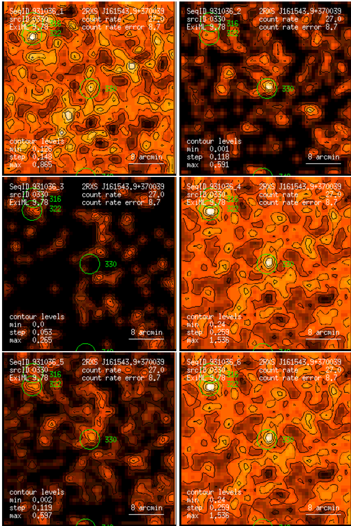
Figure 330: RASS 931036: detection 0330: band rate images, Gaussian filter: (1) PSPC channels 11 – 41, (2) 52 – 90, (3) 91 – 201, (4) 11 – 235, (5) 52 – 201, (6) 11 – 201. Broad band rates in counts/ks. Band rate contour levels in counts/ks/arcmin 2 .
