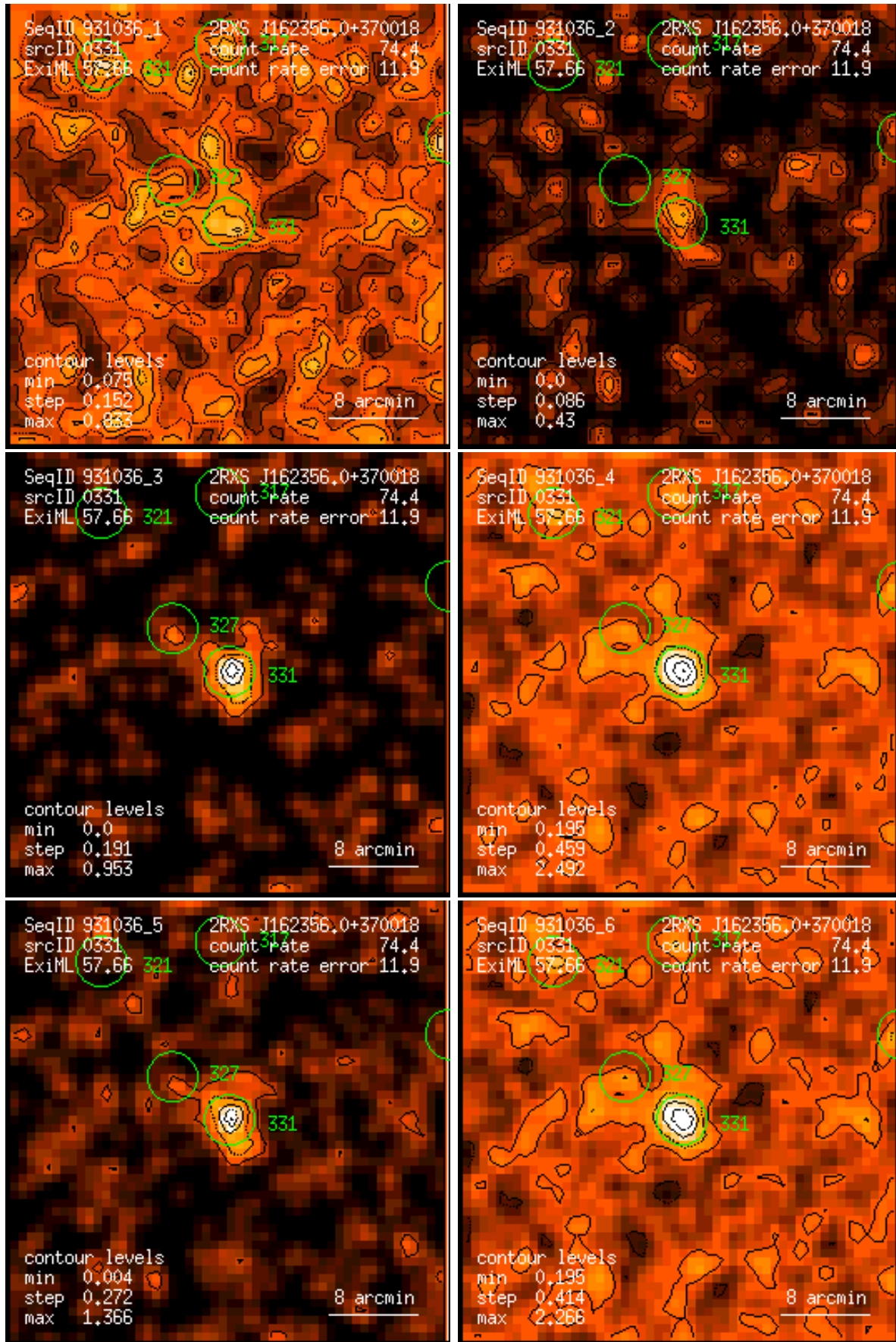
Figure 331: RASS 931036: detection 0331: band rate images, Gaussian filter: (1) PSPC channels 11 – 41, (2) 52 – 90, (3) 91 – 201, (4) 11 – 235, (5) 52 – 201, (6) 11 – 201. Broad band rates in counts/ks. Band rate contour levels in counts/ks/arcmin 2 .
