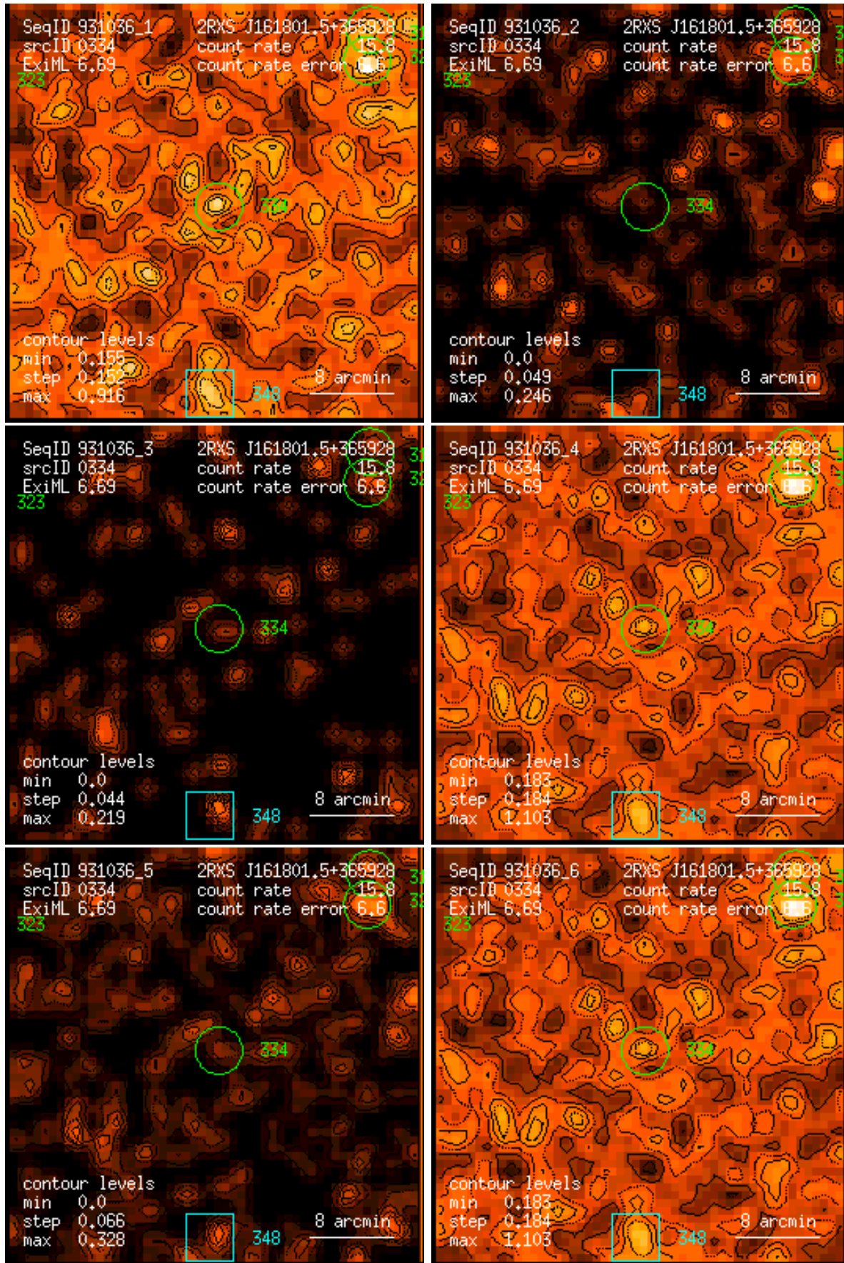
Figure 334: RASS 931036: detection 0334: band rate images, Gaussian filter: (1) PSPC channels 11 – 41, (2) 52 – 90, (3) 91 – 201, (4) 11 – 235, (5) 52 – 201, (6) 11 – 201. Broad band rates in counts/ks. Band rate contour levels in counts/ks/arcmin 2 .
