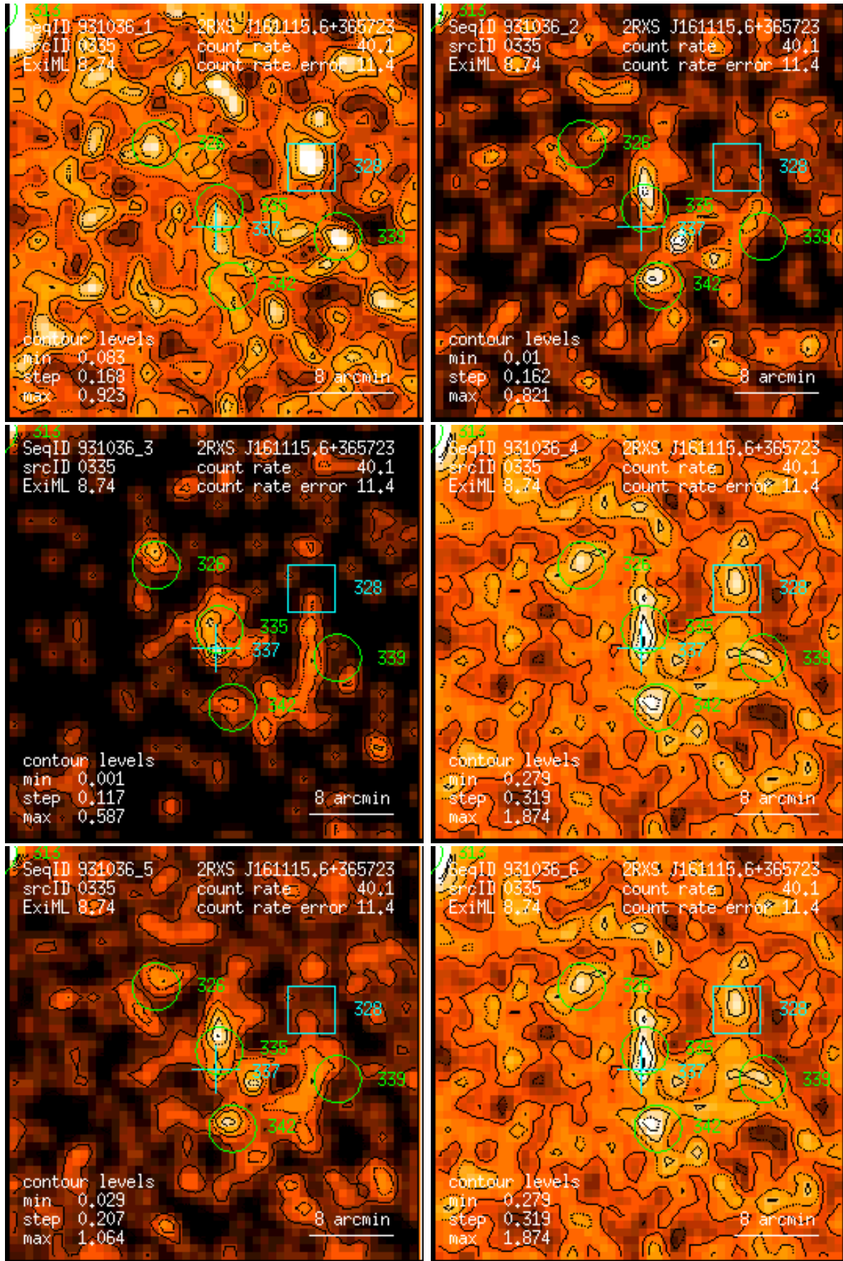
Figure 335: RASS 931036: detection 0335: band rate images, Gaussian filter: (1) PSPC channels 11 – 41, (2) 52 – 90, (3) 91 – 201, (4) 11 – 235, (5) 52 – 201, (6) 11 – 201. Broad band rates in counts/ks. Band rate contour levels in counts/ks/arcmin 2 .
