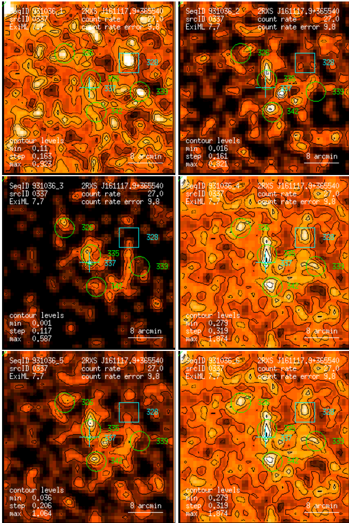
Figure 337: RASS 931036: detection 0337: band rate images, Gaussian filter: (1) PSPC channels 11 – 41, (2) 52 – 90, (3) 91 – 201, (4) 11 – 235, (5) 52 – 201, (6) 11 – 201. Broad band rates in counts/ks. Band rate contour levels in counts/ks/arcmin 2 .
