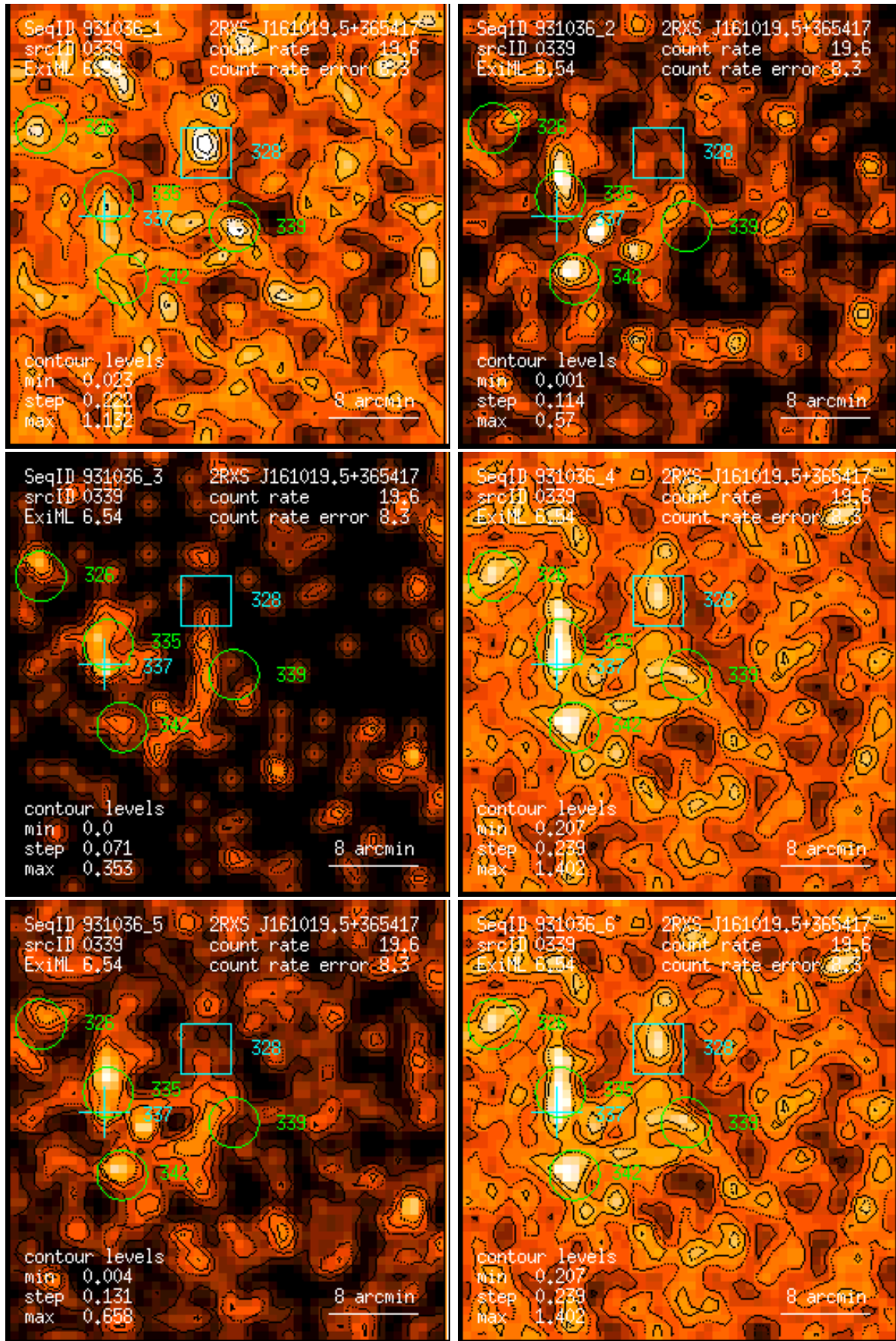
Figure 339: RASS 931036: detection 0339: band rate images, Gaussian filter: (1) PSPC channels 11 – 41, (2) 52 – 90, (3) 91 – 201, (4) 11 – 235, (5) 52 – 201, (6) 11 – 201. Broad band rates in counts/ks. Band rate contour levels in counts/ks/arcmin 2 .
