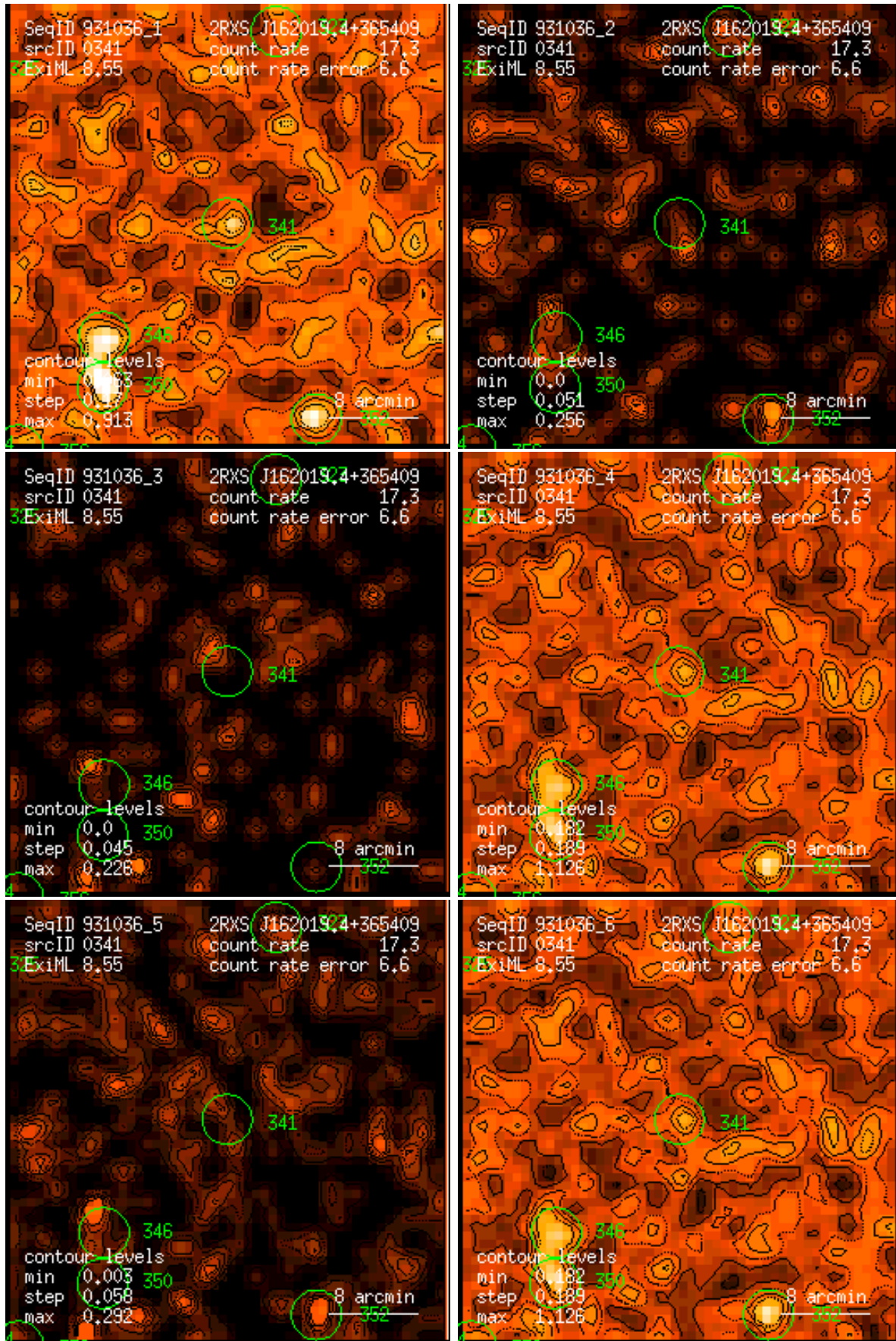
Figure 341: RASS 931036: detection 0341: band rate images, Gaussian filter: (1) PSPC channels 11 – 41, (2) 52 – 90, (3) 91 – 201, (4) 11 – 235, (5) 52 – 201, (6) 11 – 201. Broad band rates in counts/ks. Band rate contour levels in counts/ks/arcmin 2 .
