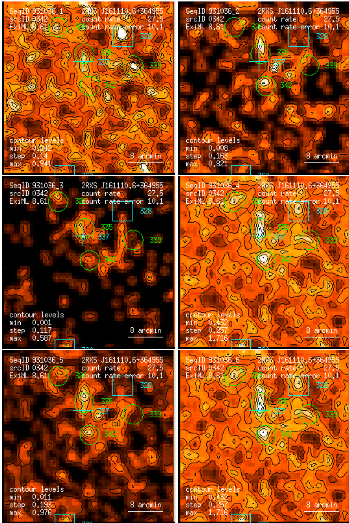
Figure 342: RASS 931036: detection 0342: band rate images, Gaussian filter: (1) PSPC channels 11 – 41, (2) 52 – 90, (3) 91 – 201, (4) 11 – 235, (5) 52 – 201, (6) 11 – 201. Broad band rates in counts/ks. Band rate contour levels in counts/ks/arcmin 2 .
