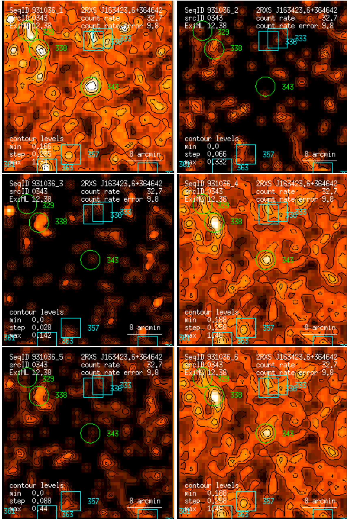
Figure 343: RASS 931036: detection 0343: band rate images, Gaussian filter: (1) PSPC channels 11 – 41, (2) 52 – 90, (3) 91 – 201, (4) 11 – 235, (5) 52 – 201, (6) 11 – 201. Broad band rates in counts/ks. Band rate contour levels in counts/ks/arcmin 2 .
