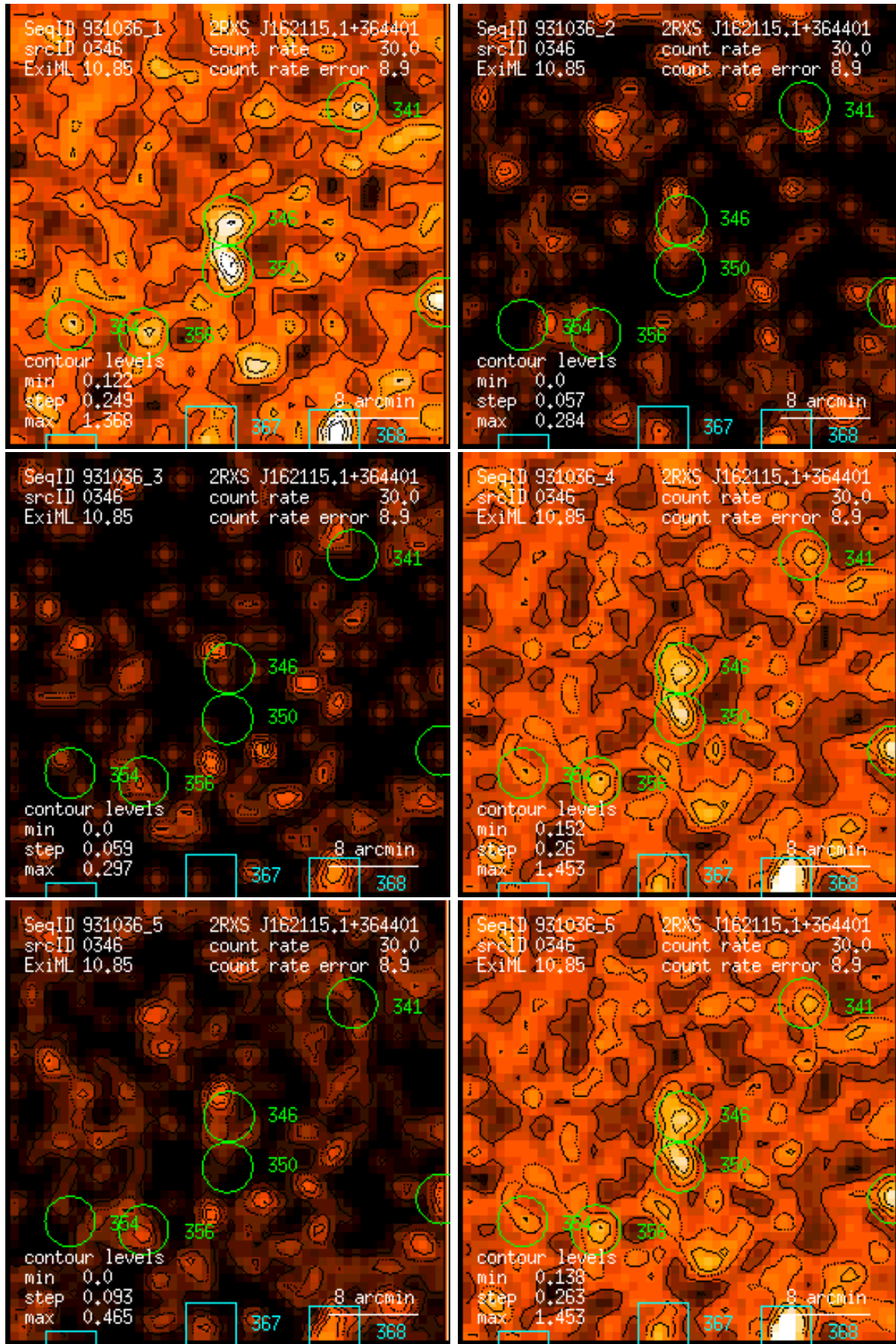
Figure 346: RASS 931036: detection 0346: band rate images, Gaussian filter: (1) PSPC channels 11 – 41, (2) 52 – 90, (3) 91 – 201, (4) 11 – 235, (5) 52 – 201, (6) 11 – 201. Broad band rates in counts/ks. Band rate contour levels in counts/ks/arcmin 2 .
