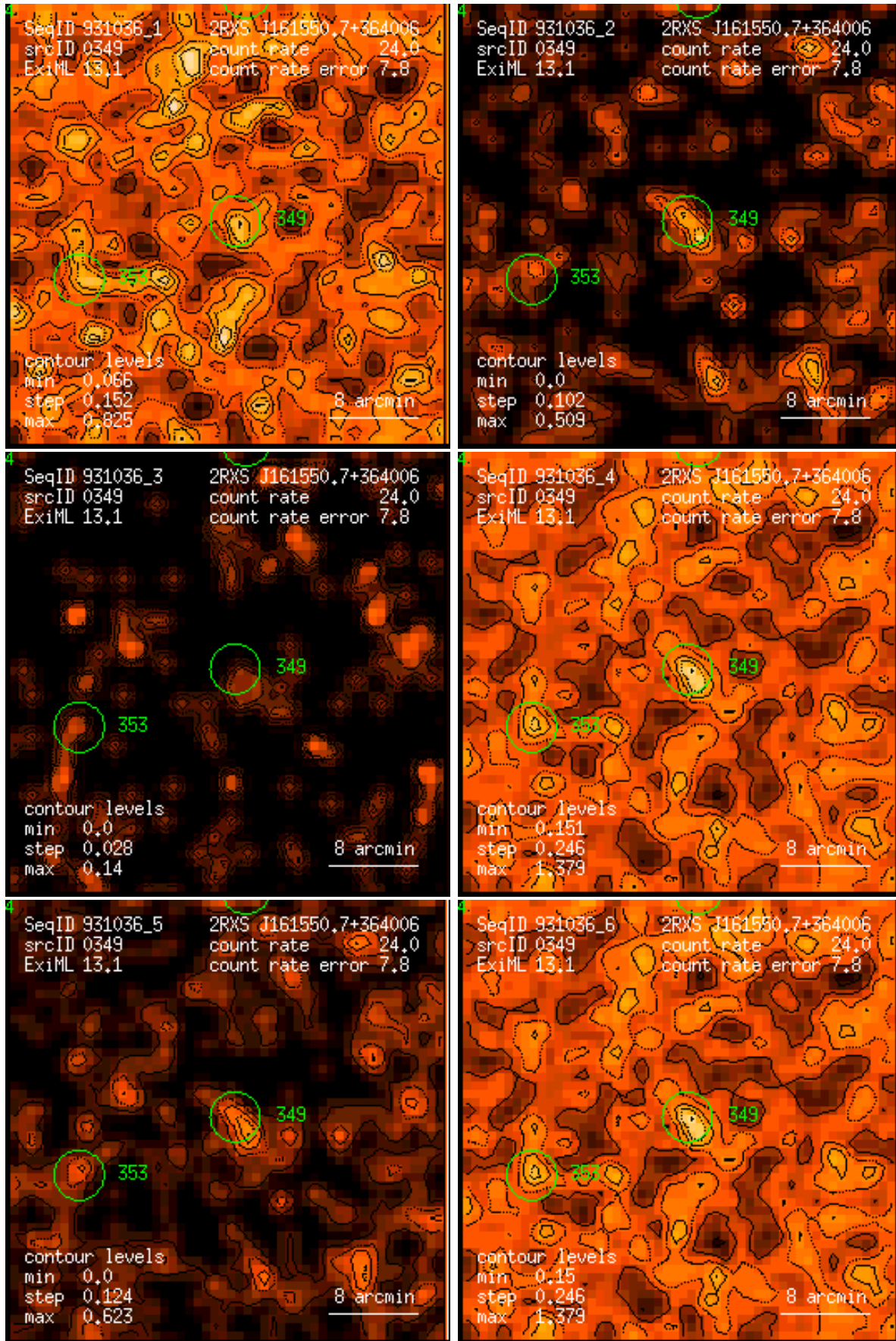
Figure 349: RASS 931036: detection 0349: band rate images, Gaussian filter: (1) PSPC channels 11 – 41, (2) 52 – 90, (3) 91 – 201, (4) 11 – 235, (5) 52 – 201, (6) 11 – 201. Broad band rates in counts/ks. Band rate contour levels in counts/ks/arcmin 2 .
