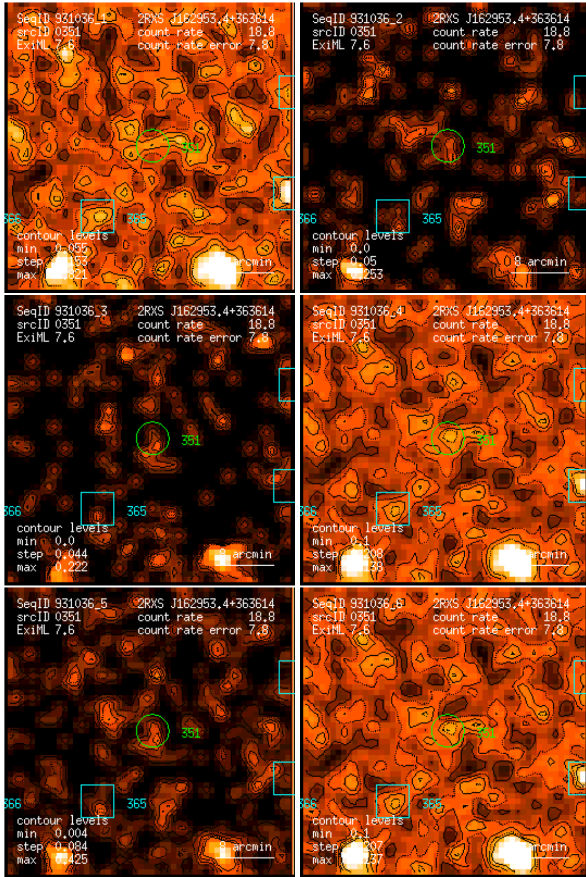
Figure 351: RASS 931036: detection 0351: band rate images, Gaussian filter: (1) PSPC channels 11 – 41, (2) 52 – 90, (3) 91 – 201, (4) 11 – 235, (5) 52 – 201, (6) 11 – 201. Broad band rates in counts/ks. Band rate contour levels in counts/ks/arcmin 2 .
