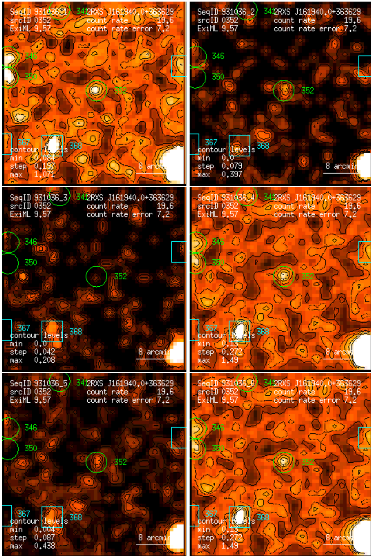
Figure 352: RASS 931036: detection 0352: band rate images, Gaussian filter: (1) PSPC channels 11 – 41, (2) 52 – 90, (3) 91 – 201, (4) 11 – 235, (5) 52 – 201, (6) 11 – 201. Broad band rates in counts/ks. Band rate contour levels in counts/ks/arcmin 2 .
