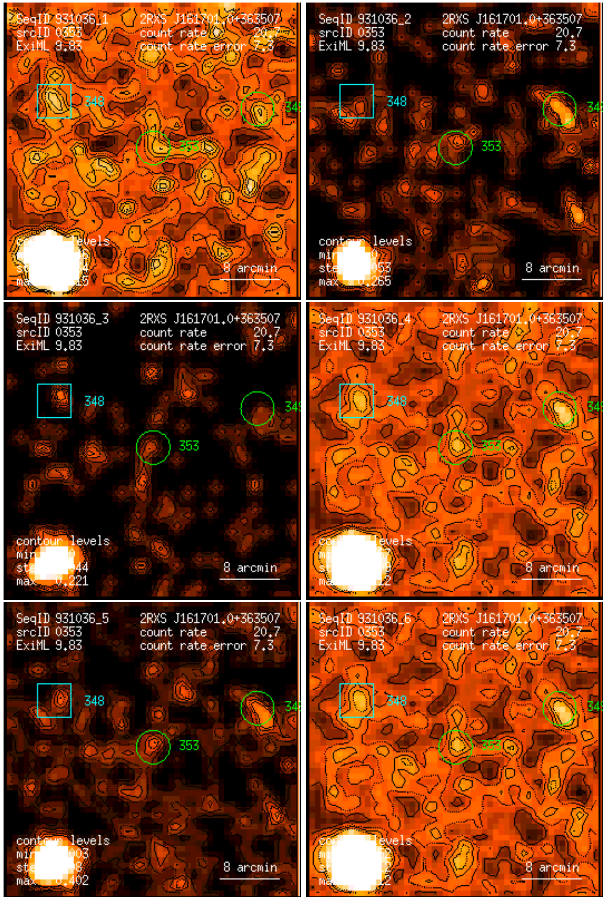
Figure 353: RASS 931036: detection 0353: band rate images, Gaussian filter: (1) PSPC channels 11 – 41, (2) 52 – 90, (3) 91 – 201, (4) 11 – 235, (5) 52 – 201, (6) 11 – 201. Broad band rates in counts/ks. Band rate contour levels in counts/ks/arcmin 2 .
