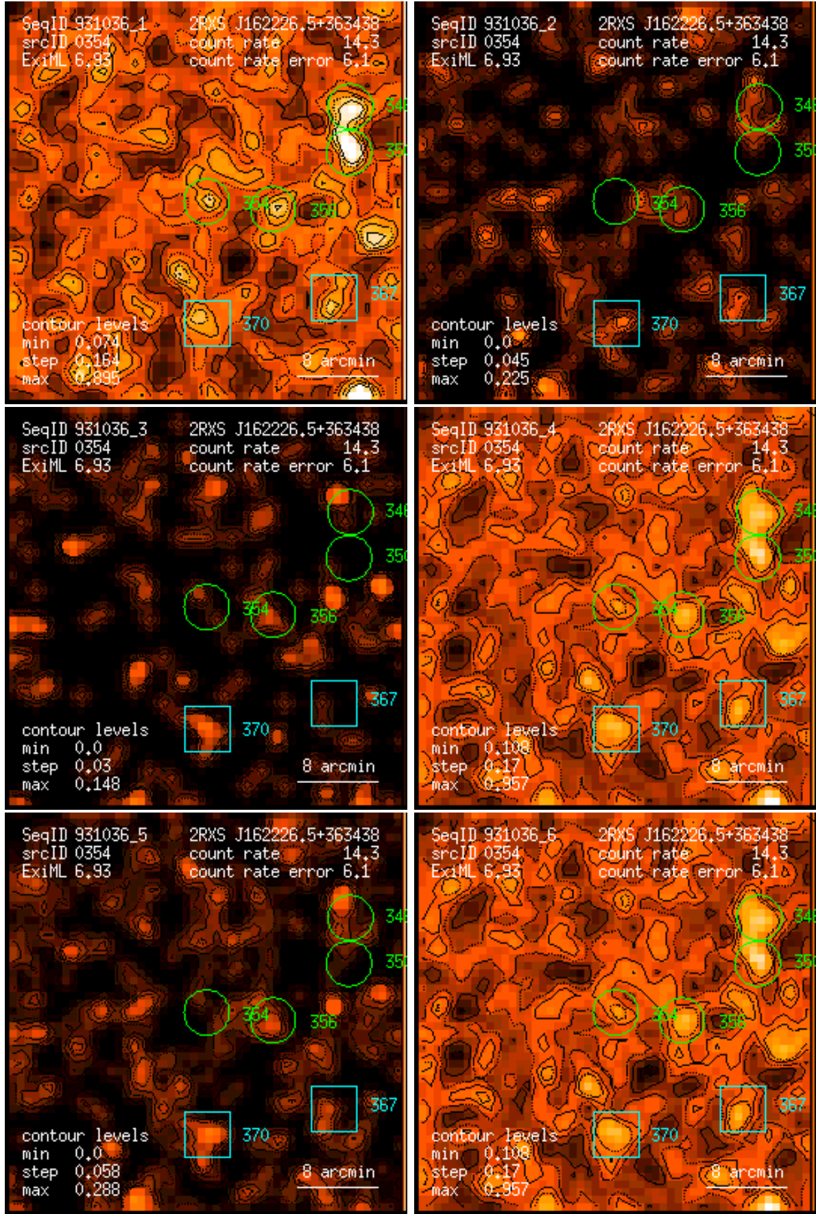
Figure 354: RASS 931036: detection 0354: band rate images, Gaussian filter: (1) PSPPC channels 11 – 41, (2) 52 – 90, (3) 91 – 201, (4) 11 – 235, (5) 52 – 201, (6) 11 – 201. Broad band rates in counts/ks. Band rate contour levels in counts/ks/arcmin 2 .
