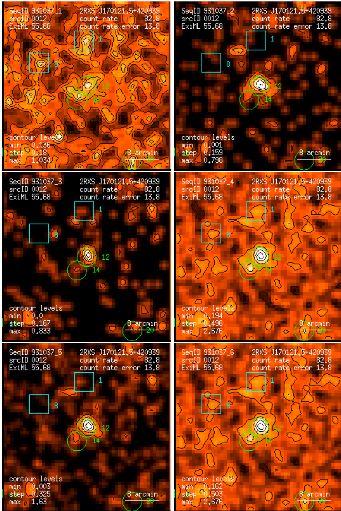
Figure 12: RASS 931037: detection 0012: band rate images, Gaussian filter: (1) PSPC channels 11 – 41, (2) 52 – 90, (3) 91 – 201, (4) 11 – 235, (5) 52 – 201, (6) 11 – 201. Broad band rates in counts/ks. Band rate contour levels in counts/ks/arcmin 2 .
