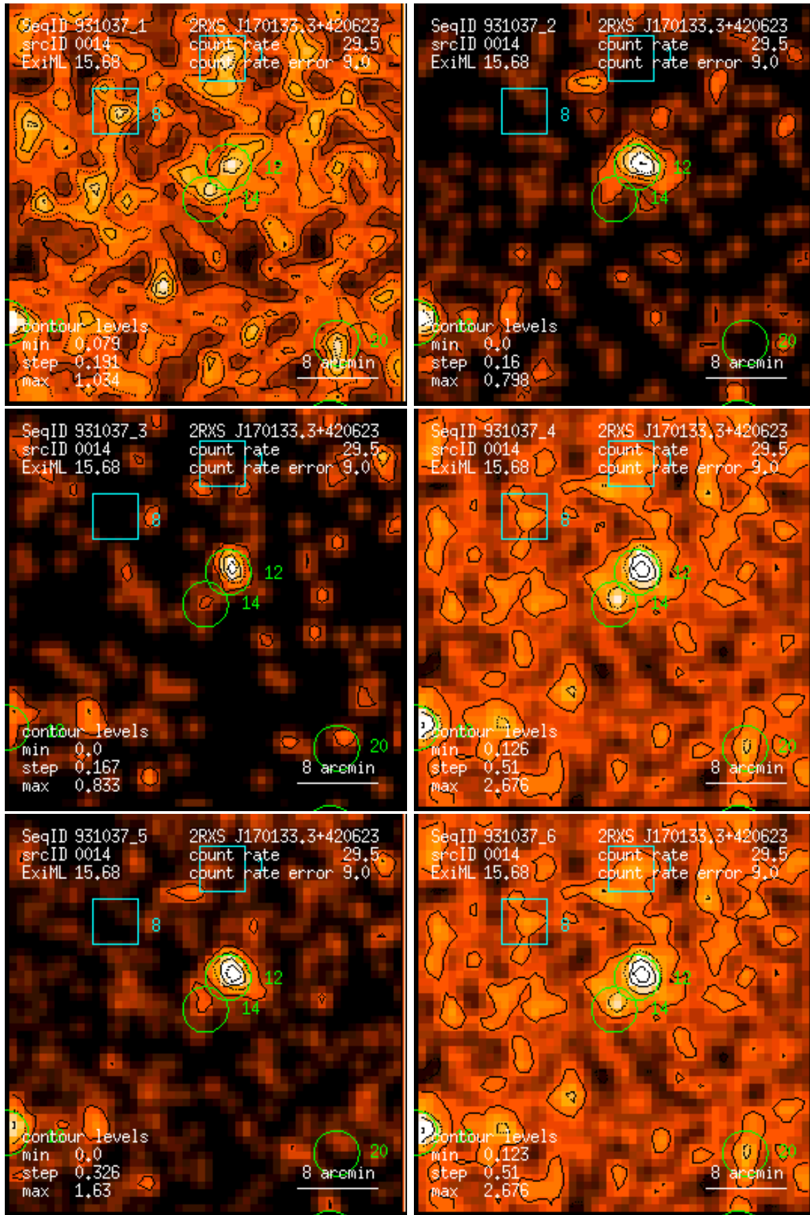
Figure 14: RASS 931037: detection 0014: band rate images, Gaussian filter: (1) PSPC channels 11 – 41, (2) 52 – 90, (3) 91 – 201, (4) 11 – 235, (5) 52 – 201, (6) 11 – 201. Broad band rates in counts/ks. Band rate contour levels in counts/ks/arcmin 2 .
