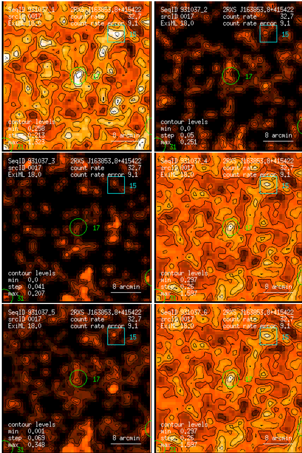
Figure 17: RASS 931037: detection 0017: band rate images, Gaussian filter: (1) PSPC channels 11 – 41, (2) 52 – 90, (3) 91 – 201, (4) 11 – 235, (5) 52 – 201, (6) 11 – 201. Broad band rates in counts/ks. Band rate contour levels in counts/ks/arcmin 2 .
