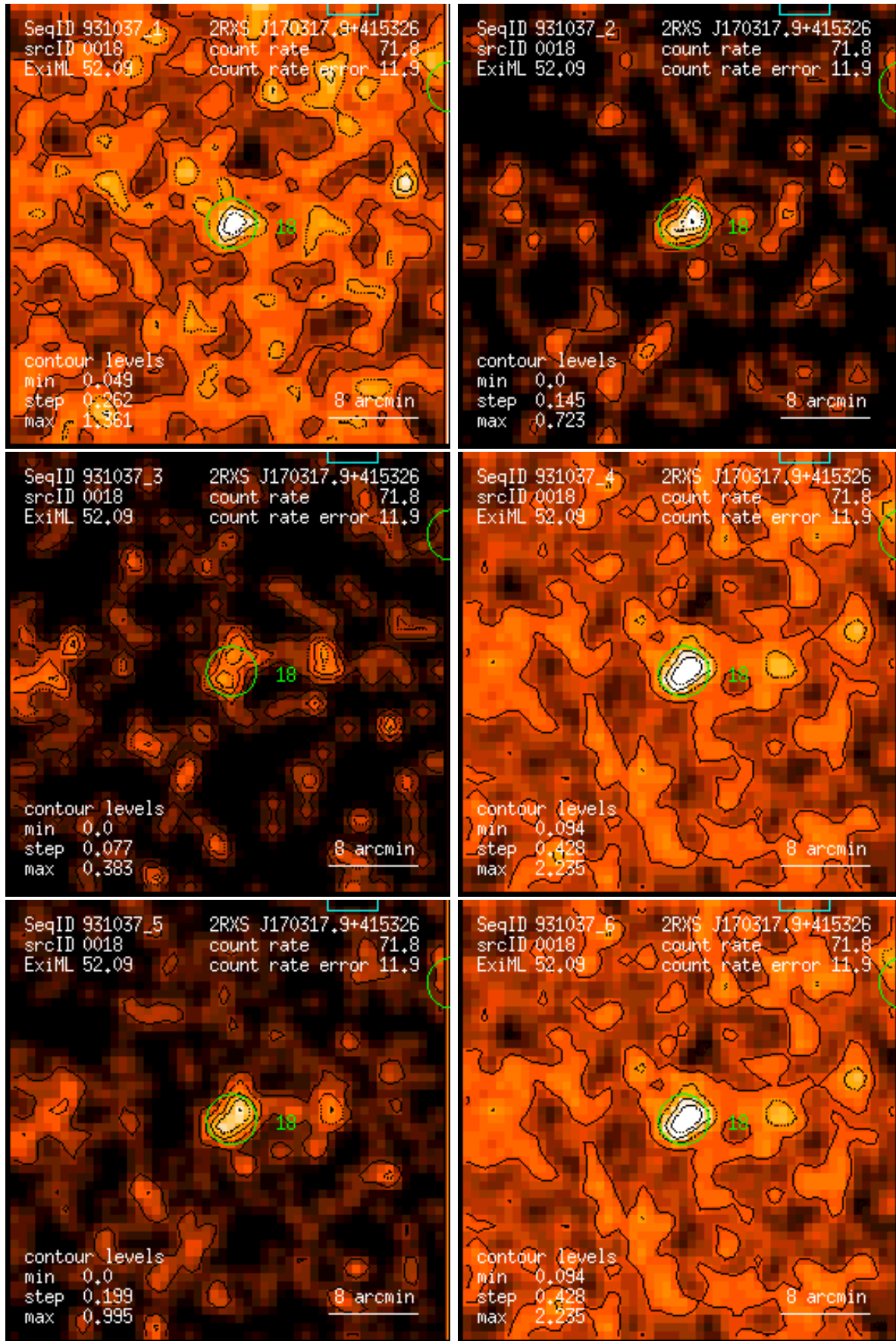
Figure 18: RASS 931037: detection 0018: band rate images, Gaussian filter: (1) PSPC channels 11 – 41, (2) 52 – 90, (3) 91 – 201, (4) 11 – 235, (5) 52 – 201, (6) 11 – 201. Broad band rates in counts/ks. Band rate contour levels in counts/ks/arcmin 2 .
